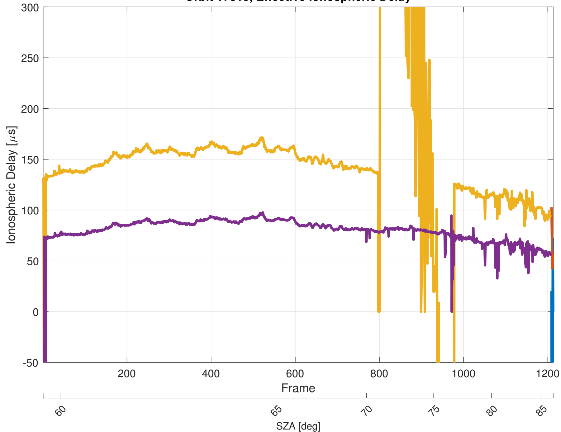
Orbit 17815, Effective Ionospheric Delay
