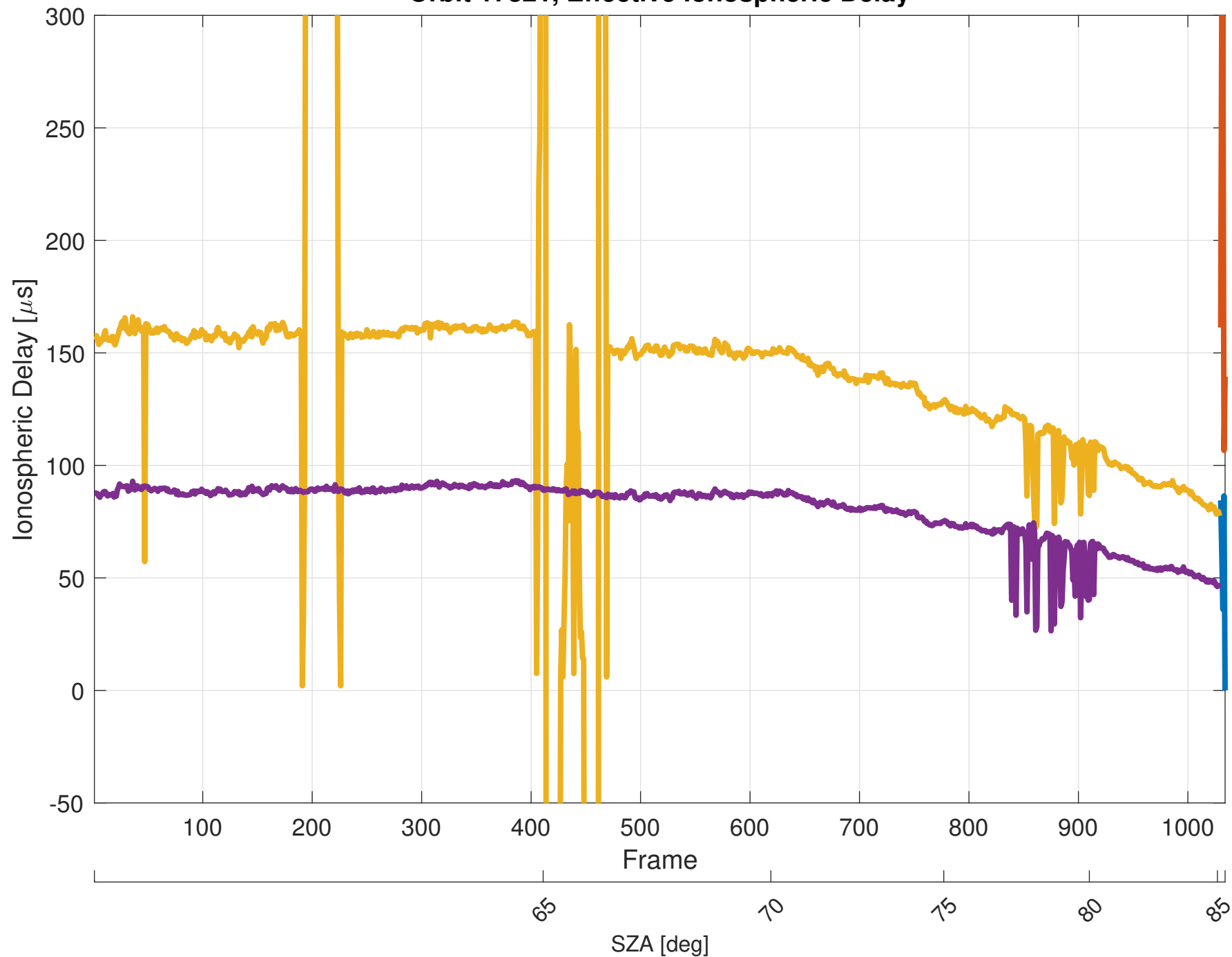
Orbit 17821, Effective Ionospheric Delay
