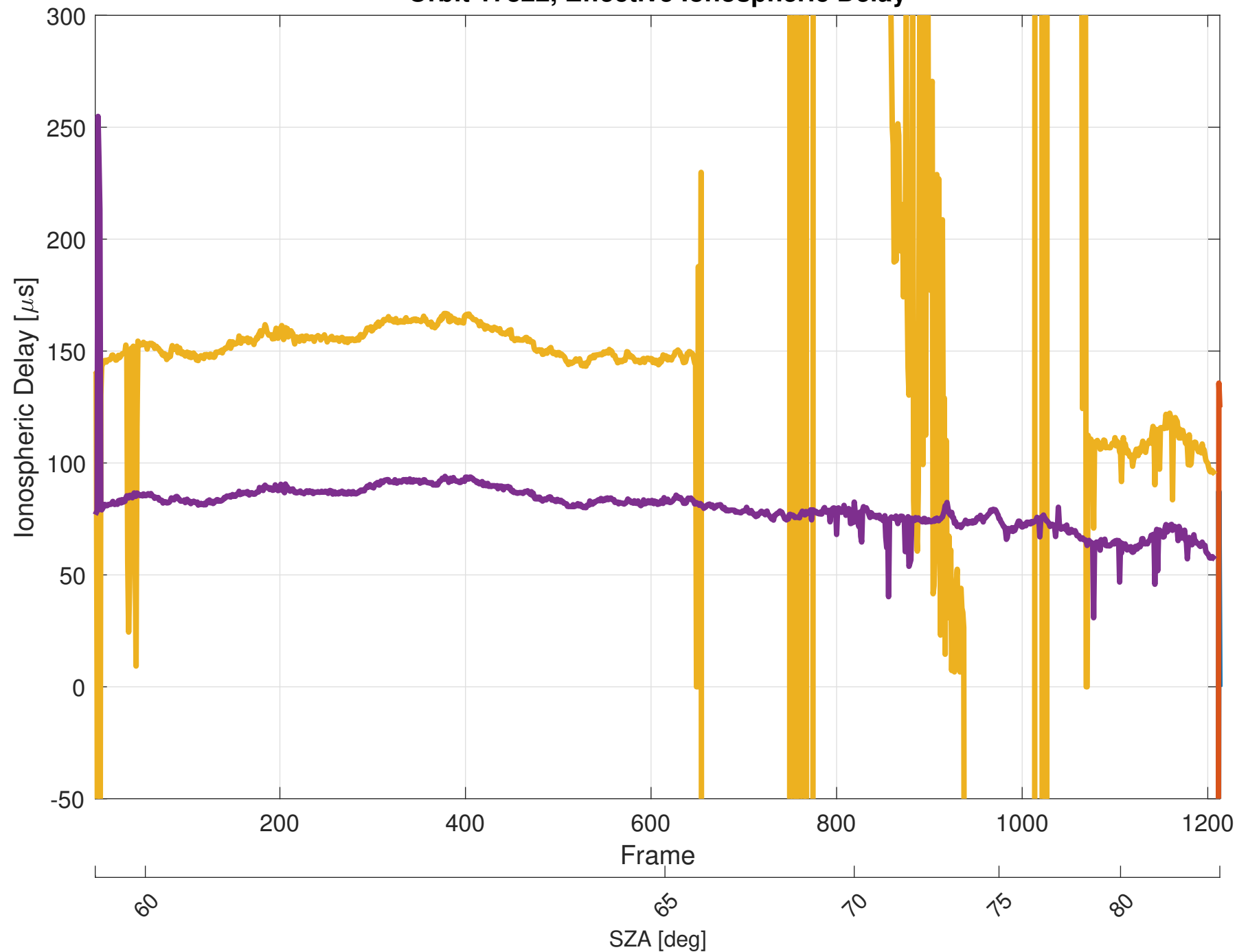
Orbit 17822, Effective Ionospheric Delay
