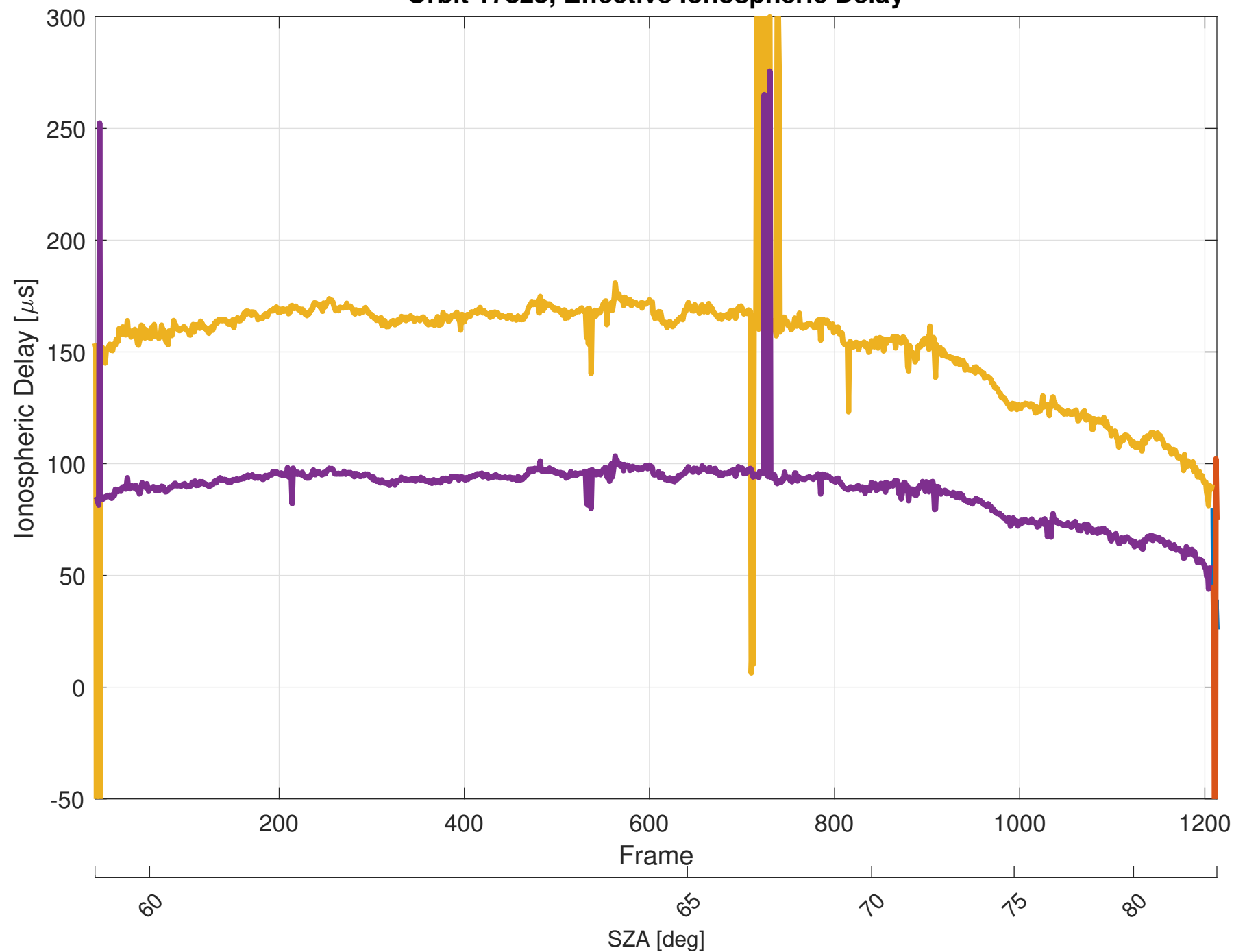
Orbit 17825, Effective Ionospheric Delay
