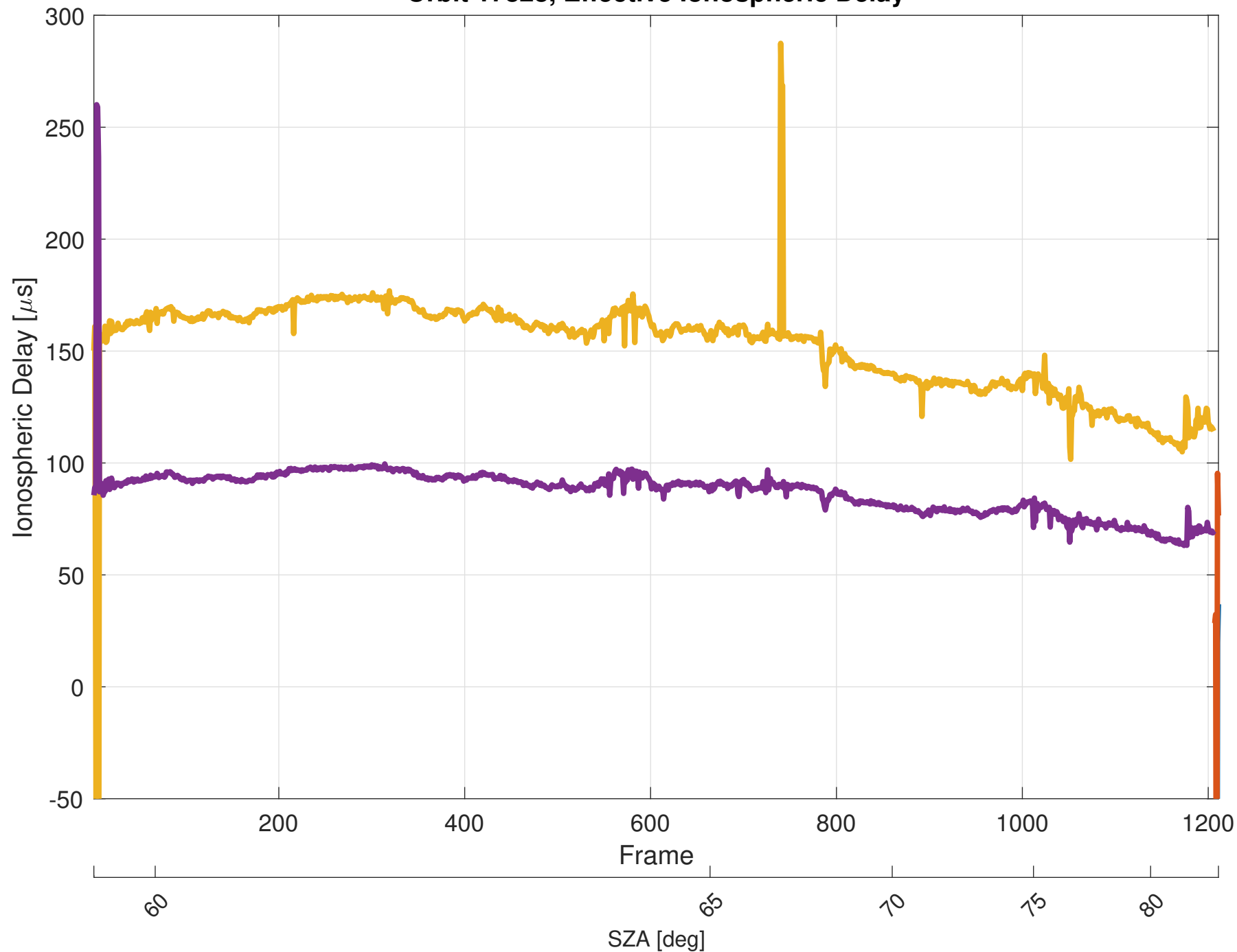
Orbit 17828, Effective Ionospheric Delay
