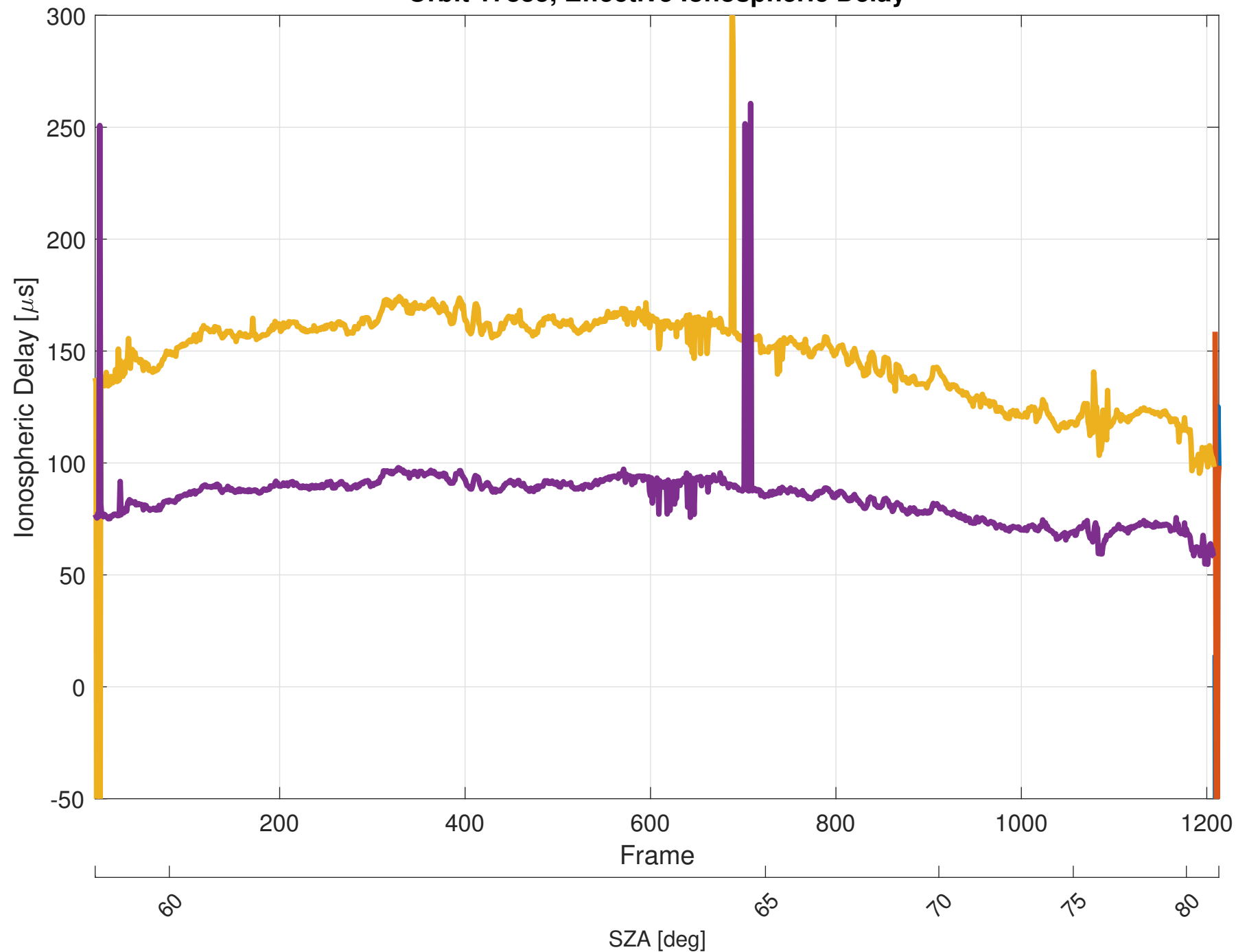
Orbit 17835, Effective Ionospheric Delay
