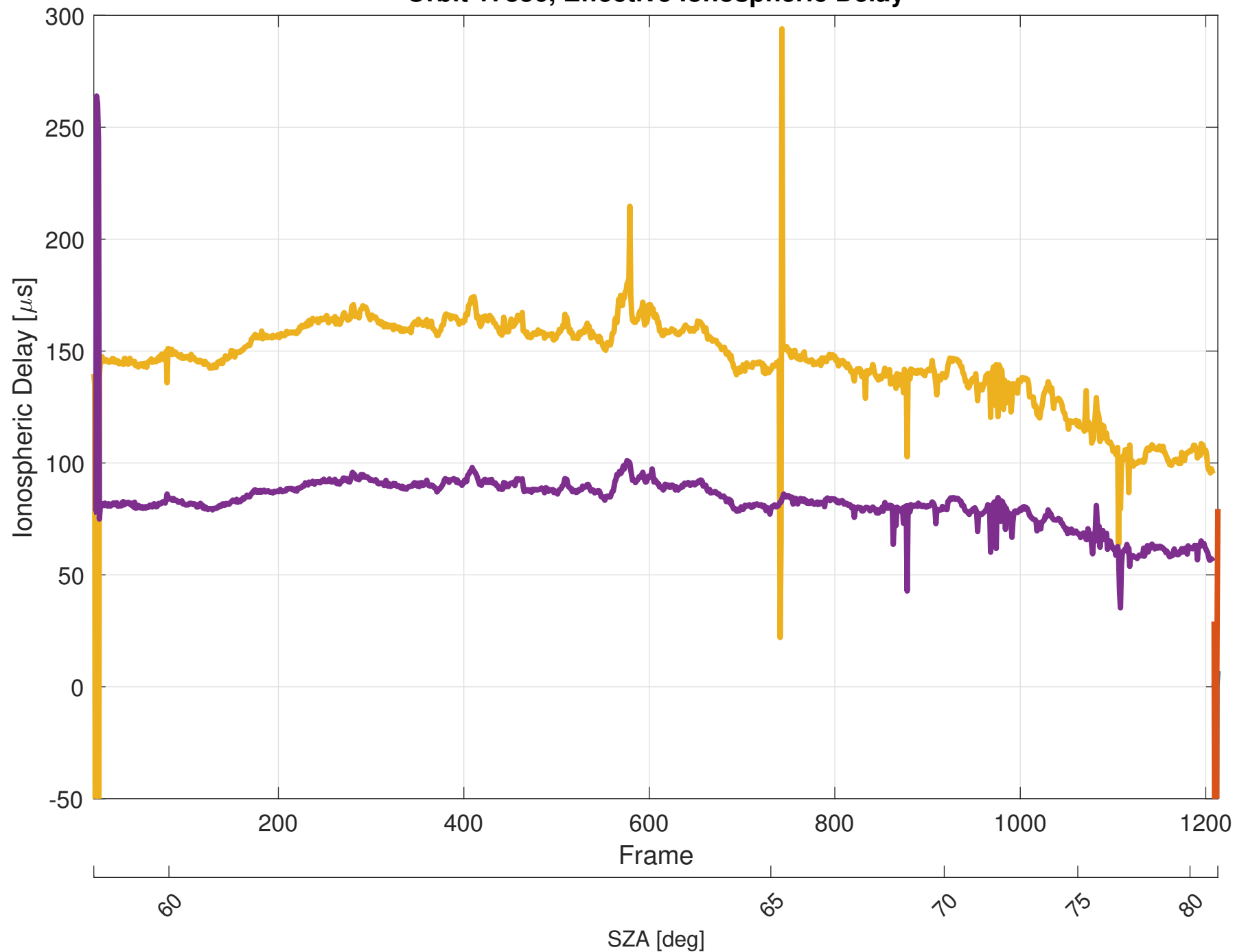
Orbit 17836, Effective Ionospheric Delay
