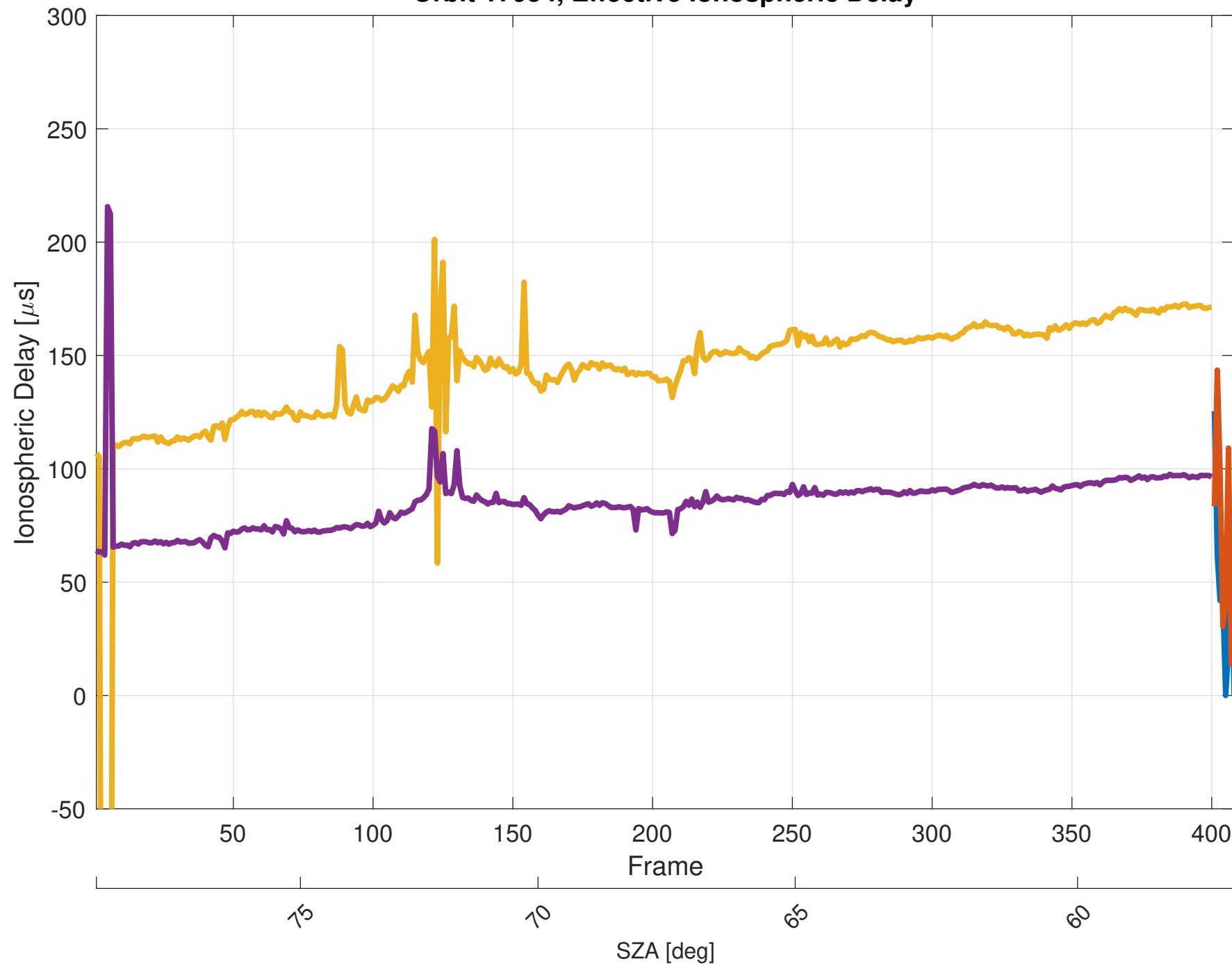
Orbit 17954, Effective Ionospheric Delay
