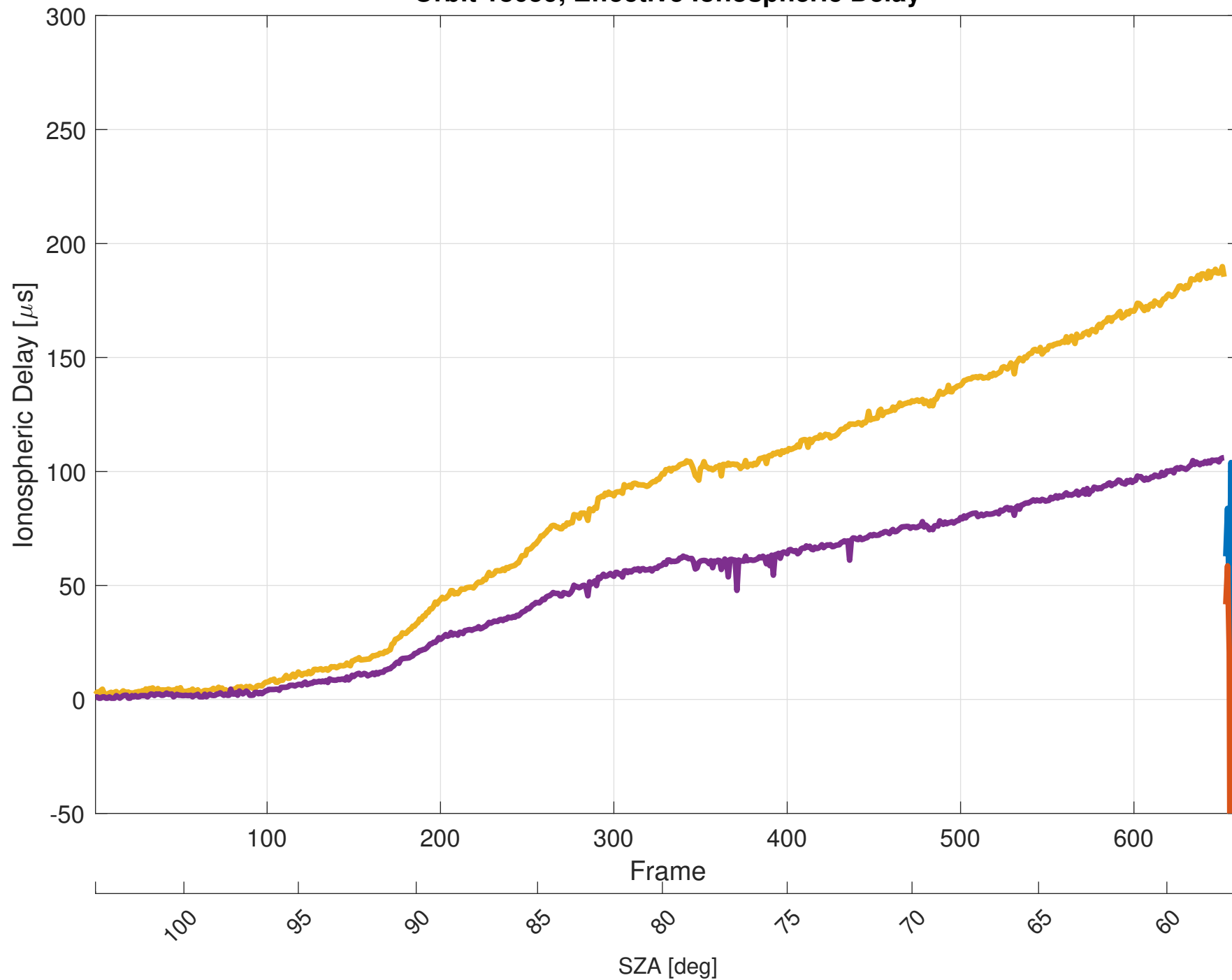
Orbit 18059, Effective Ionospheric Delay
