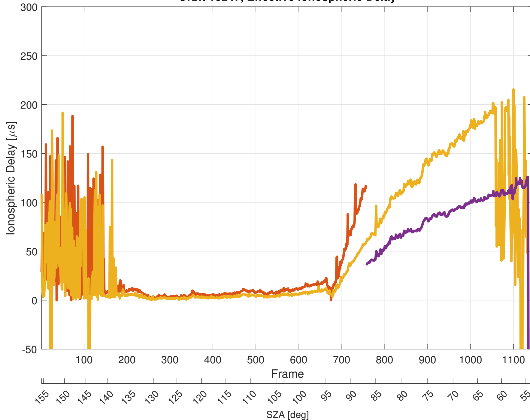
Orbit 18247, Effective Ionospheric Delay
