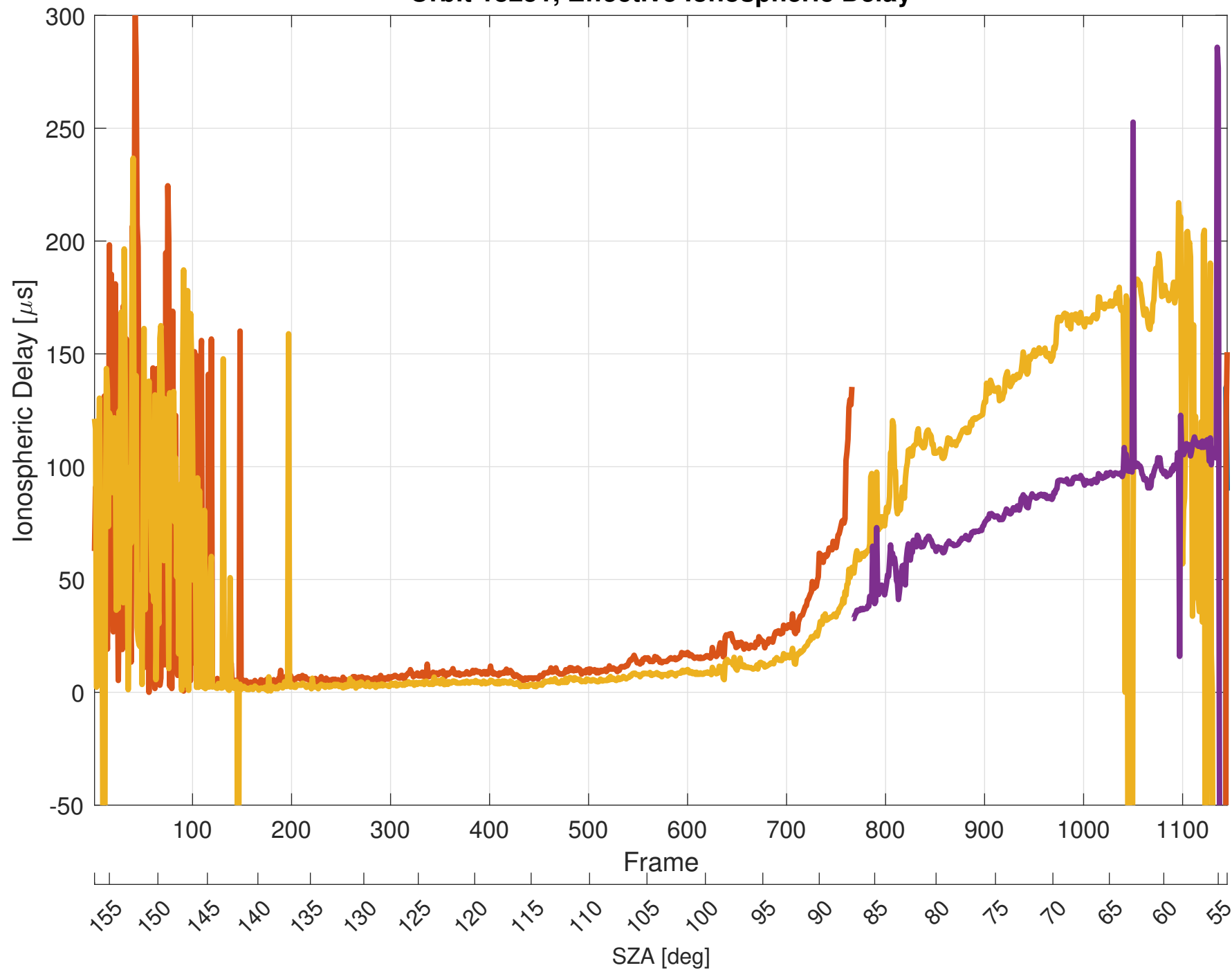
Orbit 18251, Effective Ionospheric Delay
