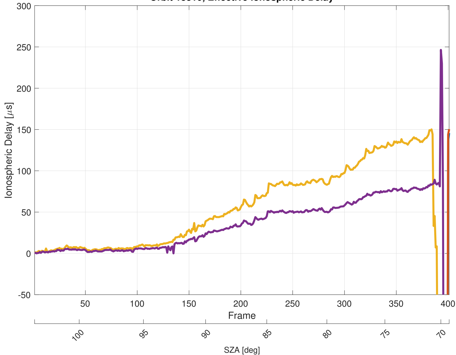
Orbit 18310, Effective Ionospheric Delay
