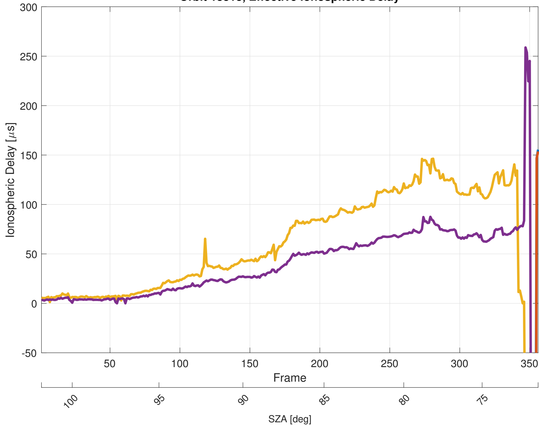
Orbit 18318, Effective Ionospheric Delay
