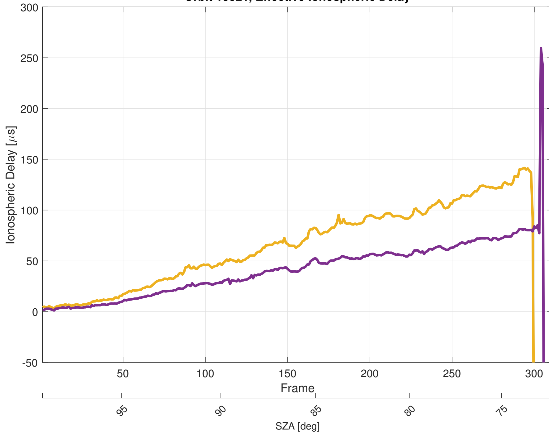
Orbit 18321, Effective Ionospheric Delay
