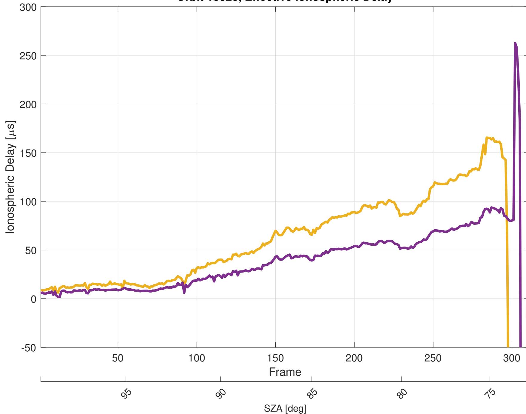
Orbit 18323, Effective Ionospheric Delay
