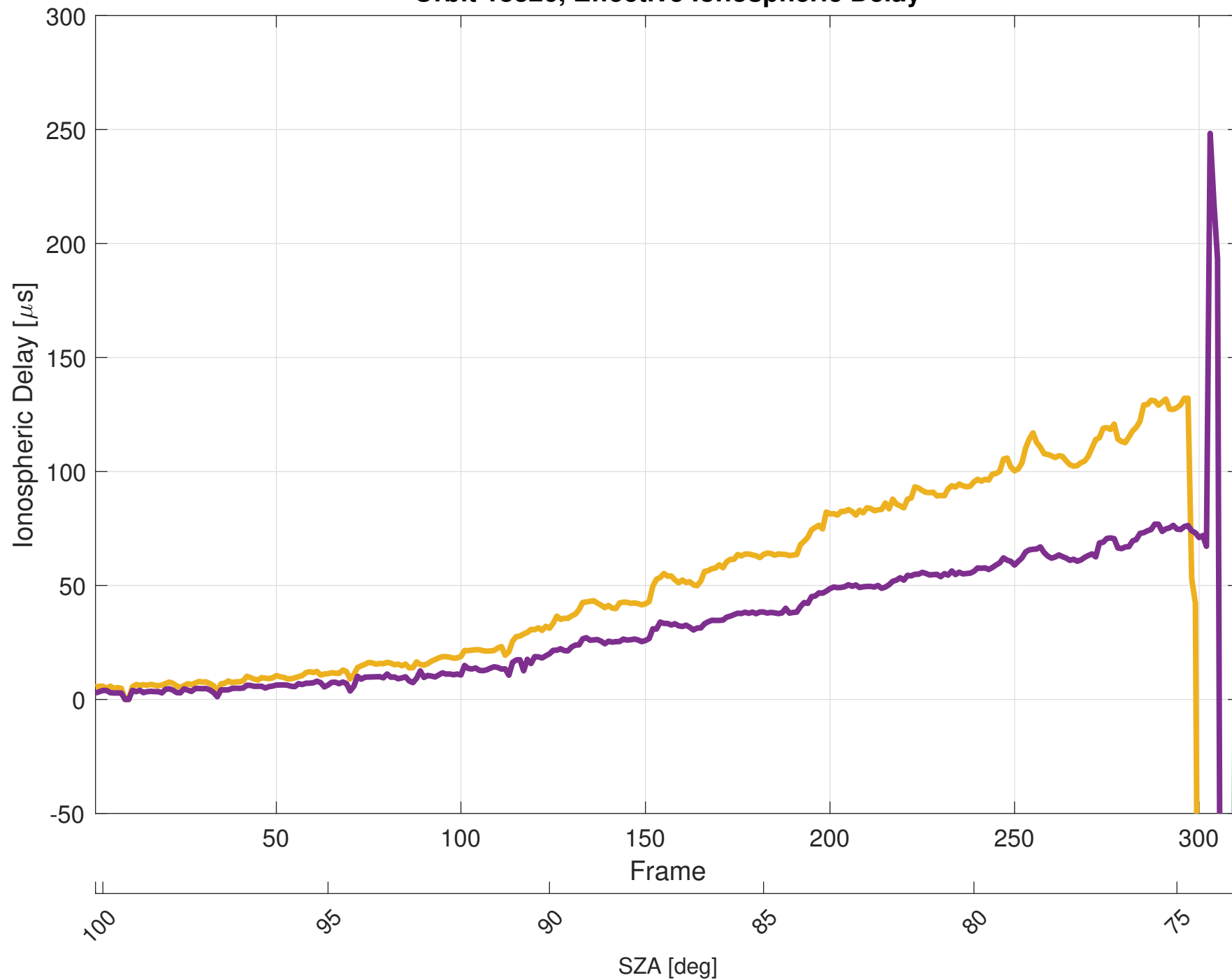
Orbit 18326, Effective Ionospheric Delay
