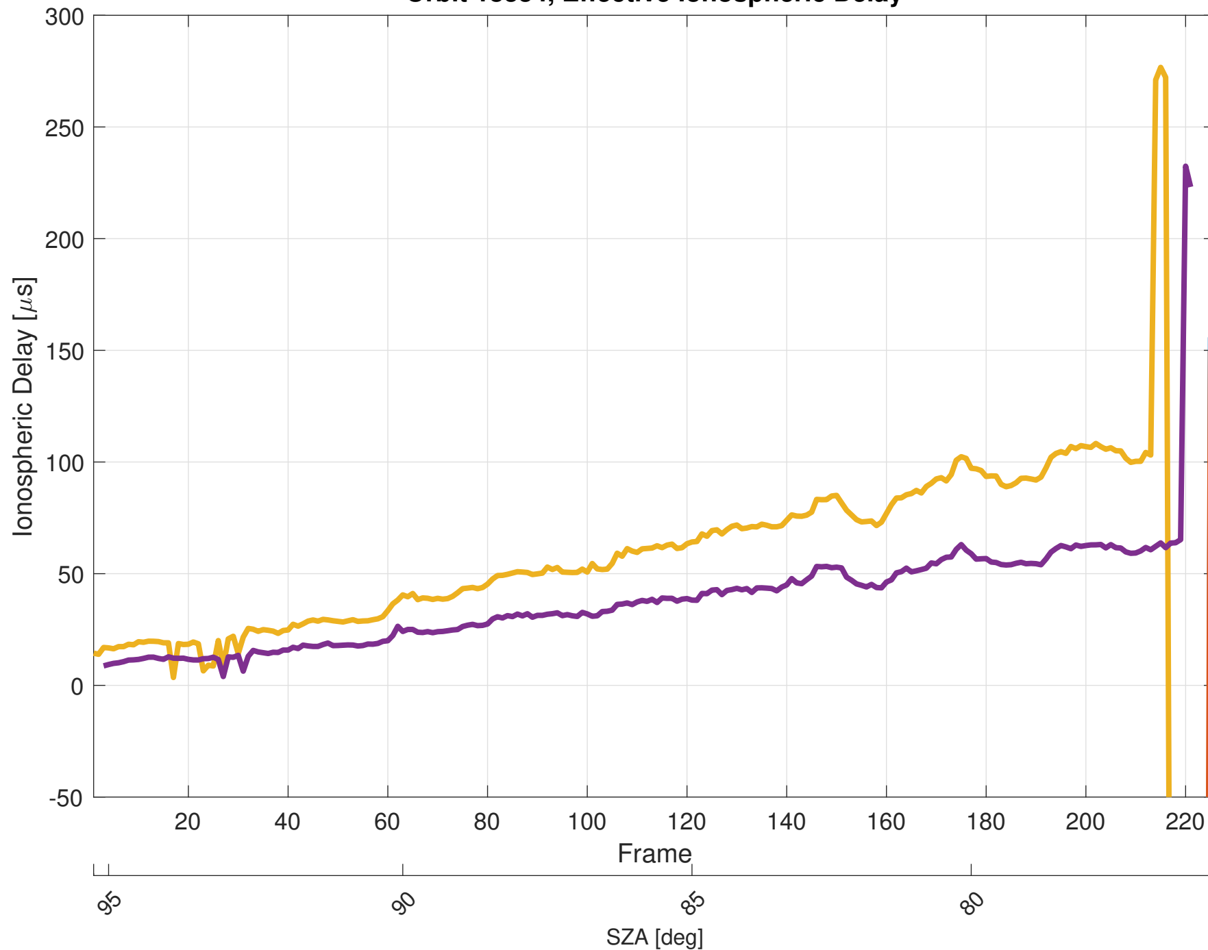
Orbit 18334, Effective Ionospheric Delay
