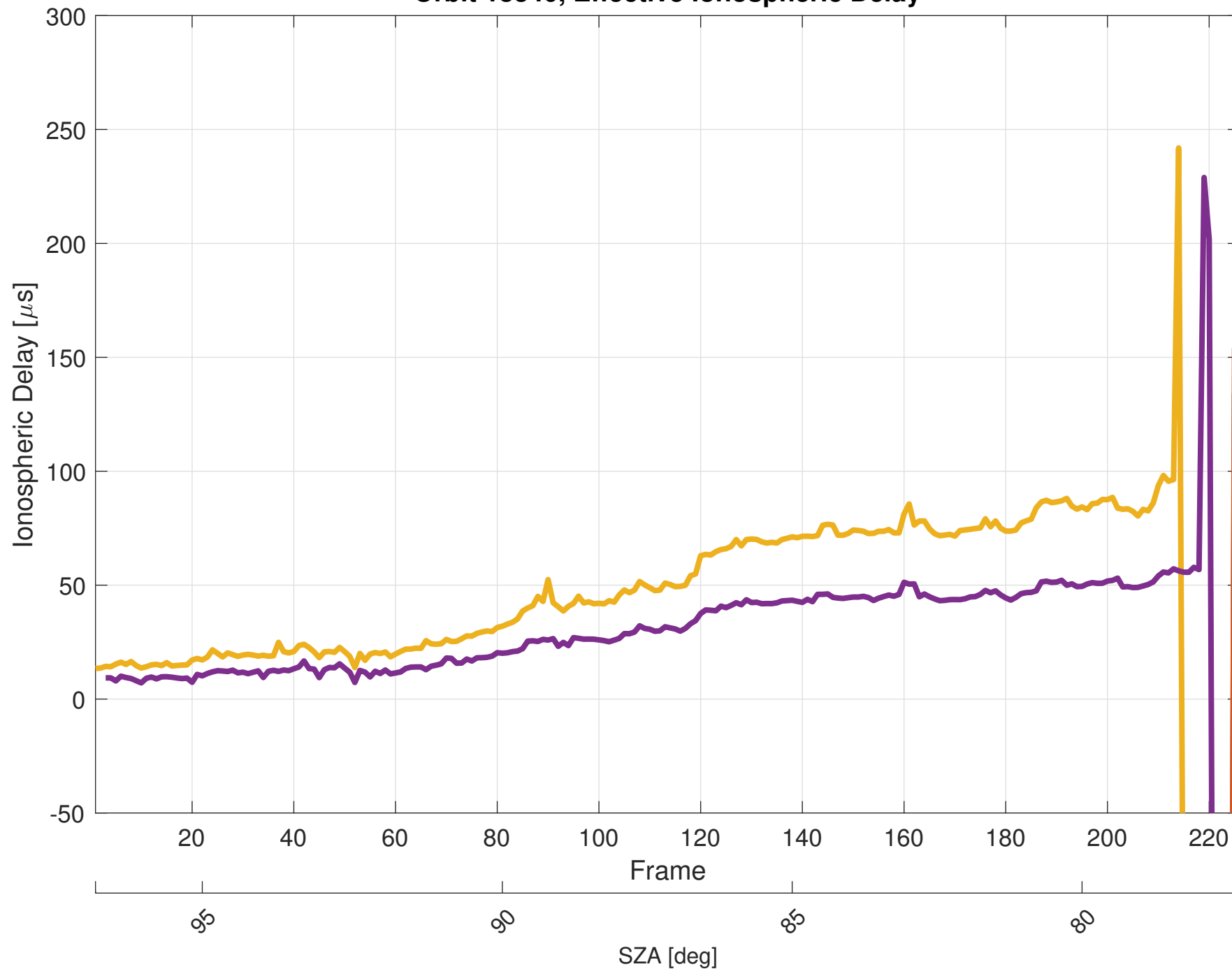
Orbit 18340, Effective Ionospheric Delay
