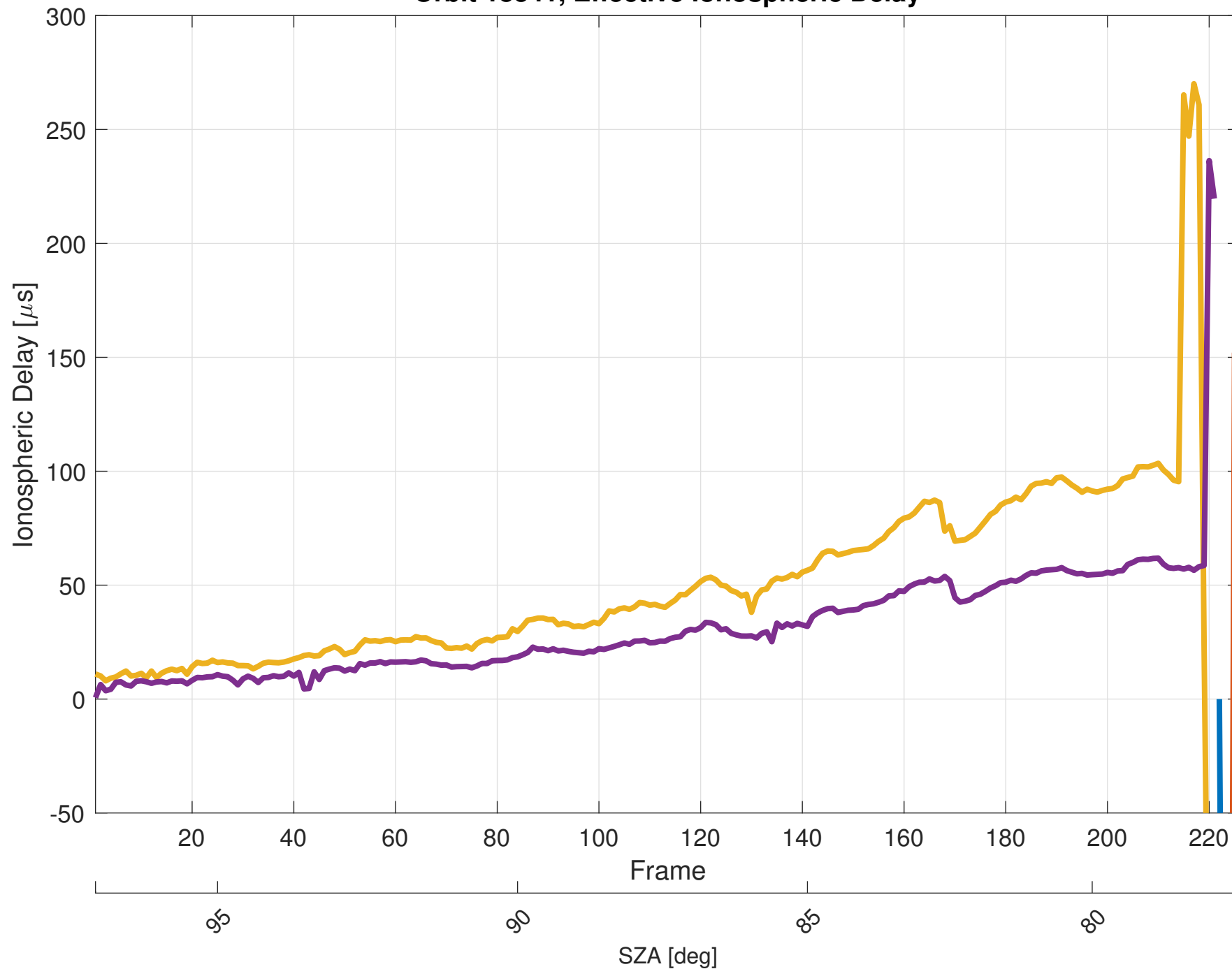
Orbit 18341, Effective Ionospheric Delay
