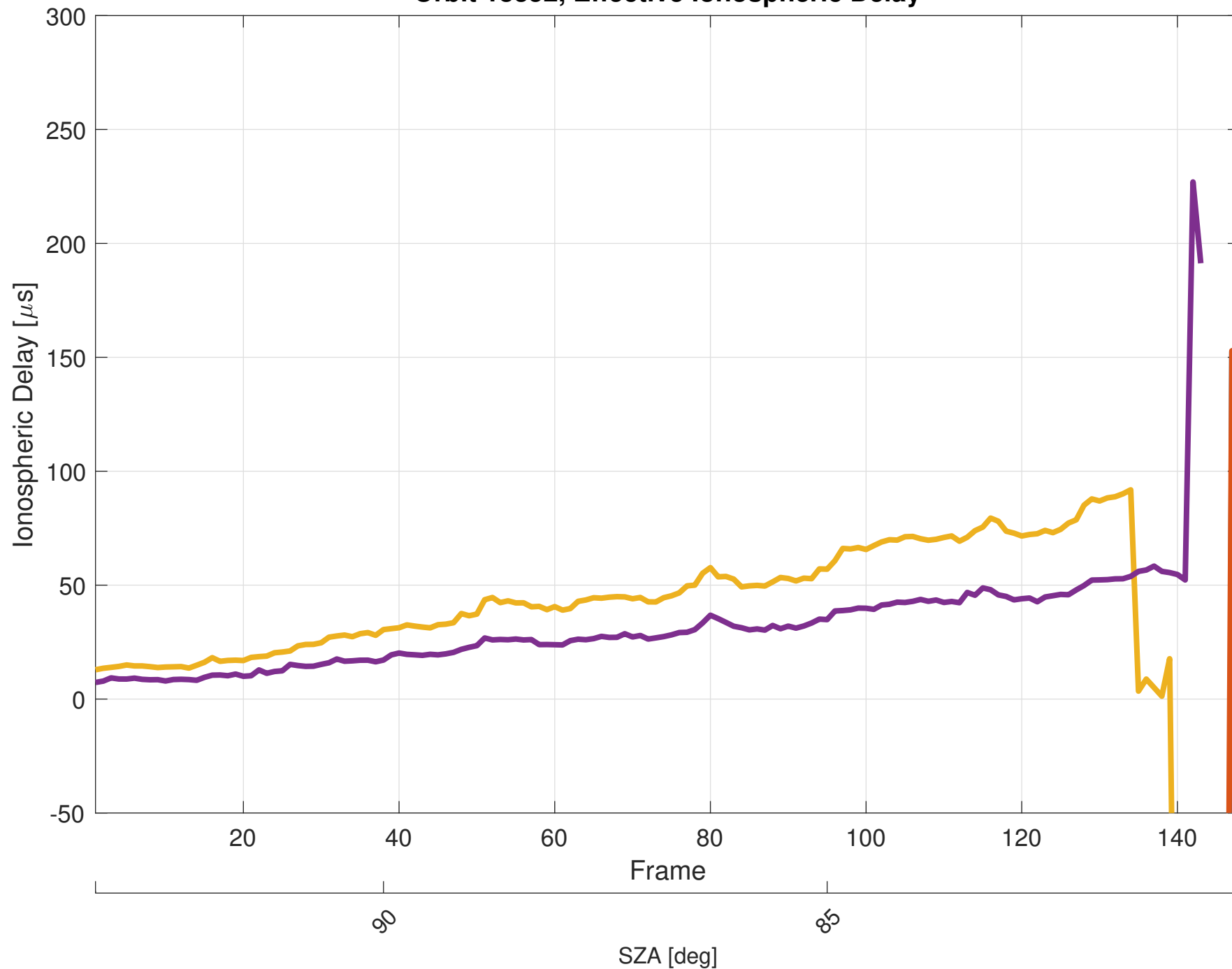
Orbit 18352, Effective Ionospheric Delay
