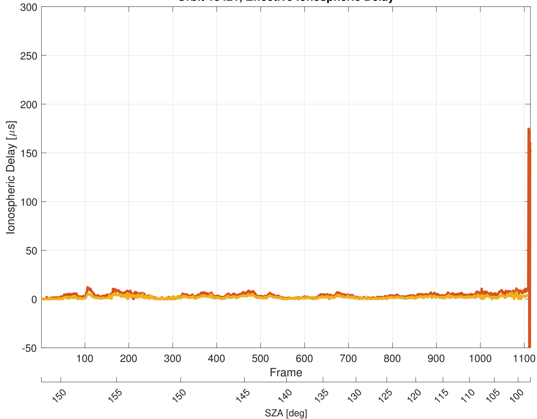
Orbit 18421, Effective Ionospheric Delay
