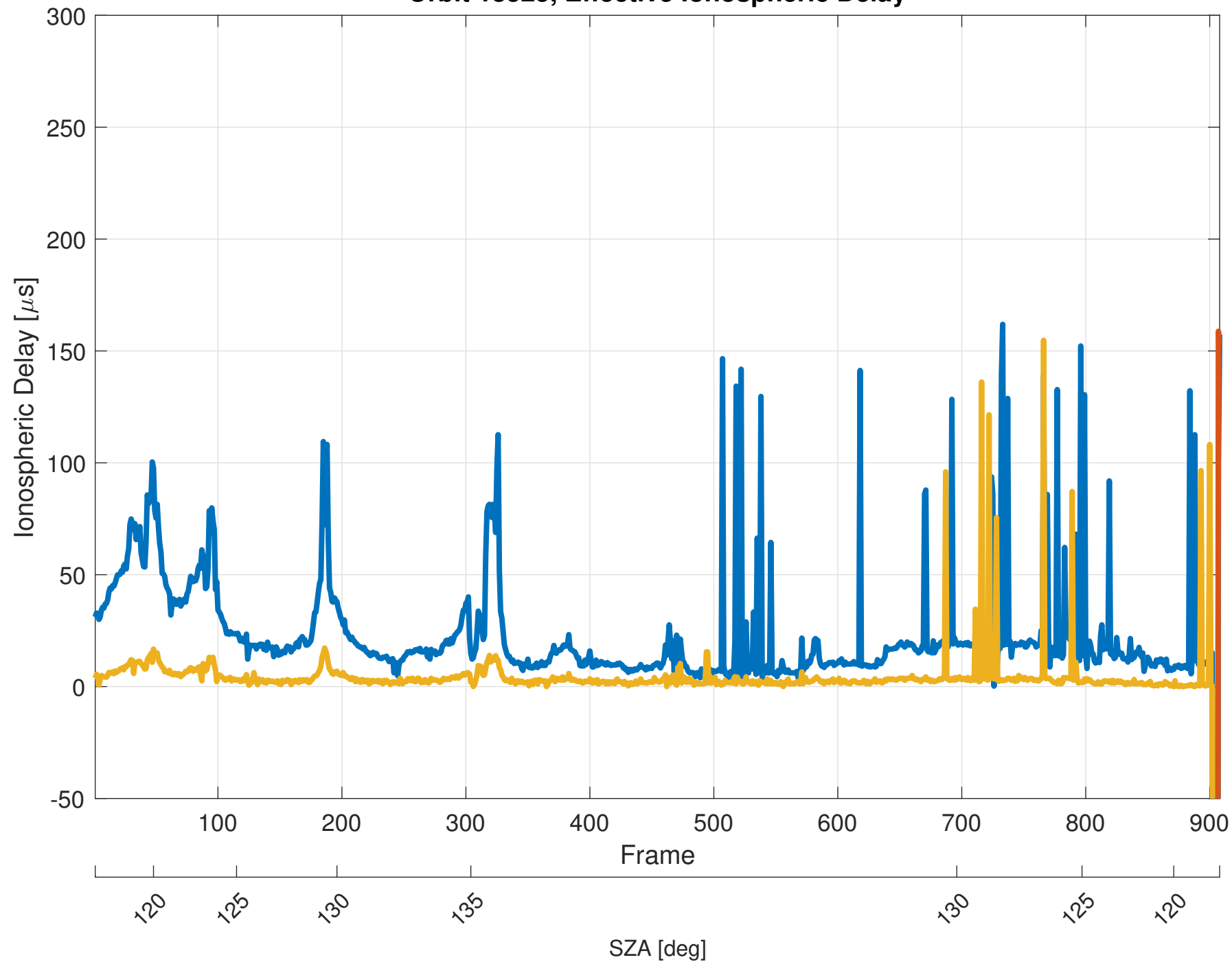
Orbit 18525, Effective Ionospheric Delay
