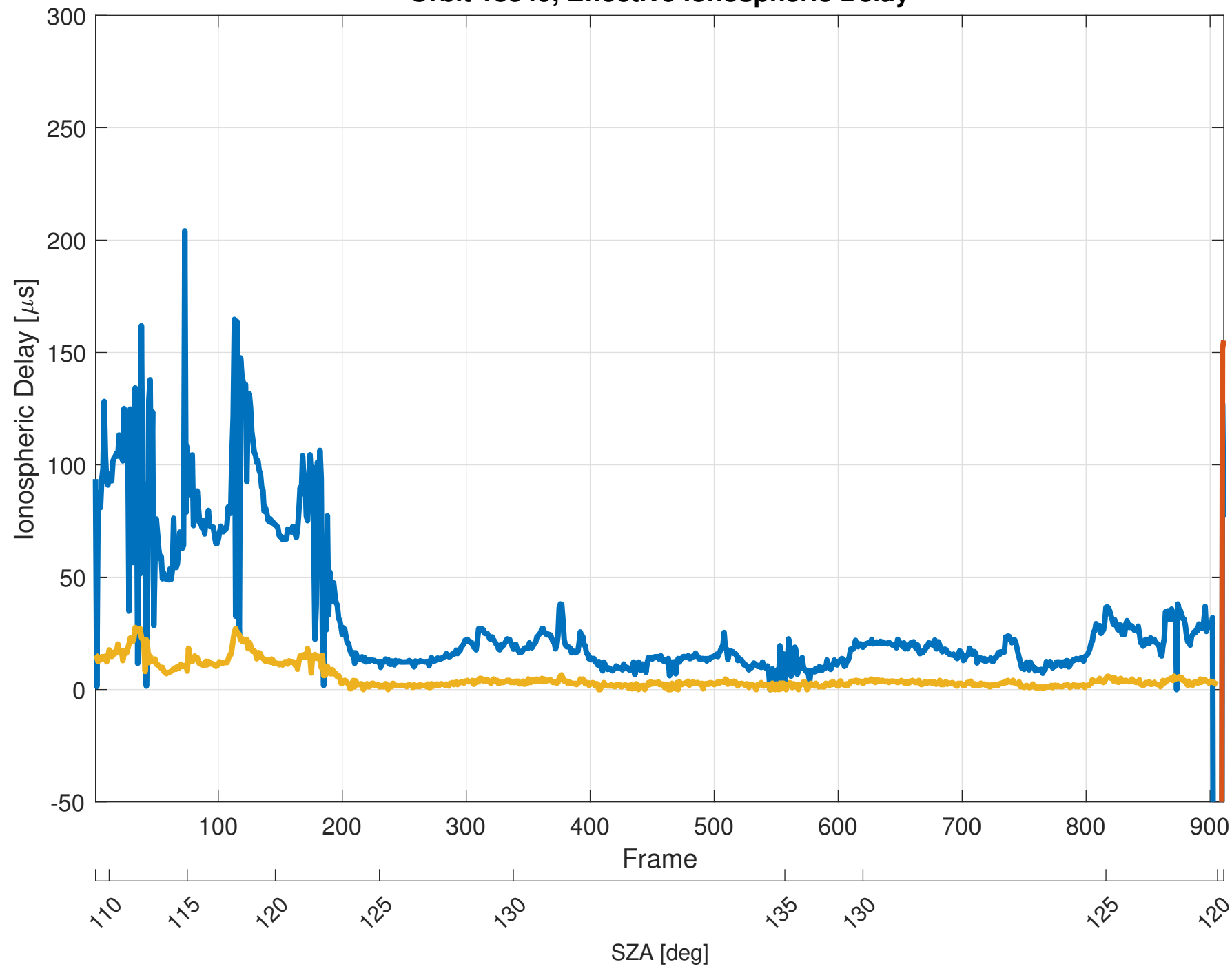
Orbit 18549, Effective Ionospheric Delay
