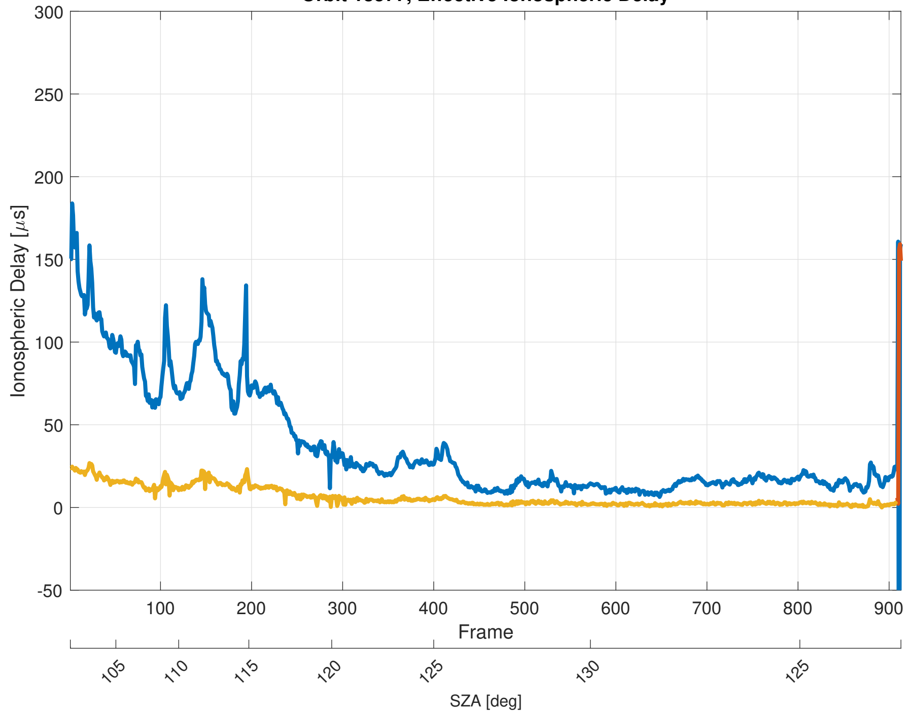
Orbit 18577, Effective Ionospheric Delay
