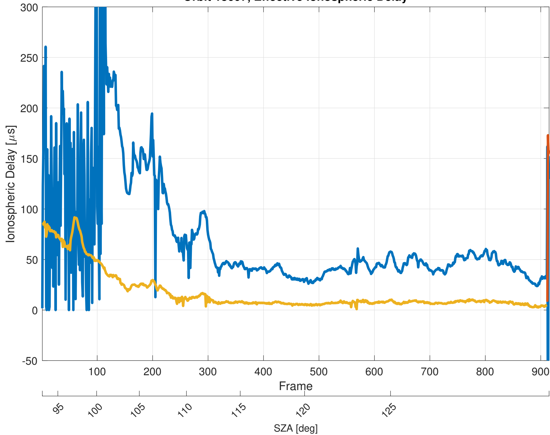
Orbit 18607, Effective Ionospheric Delay
