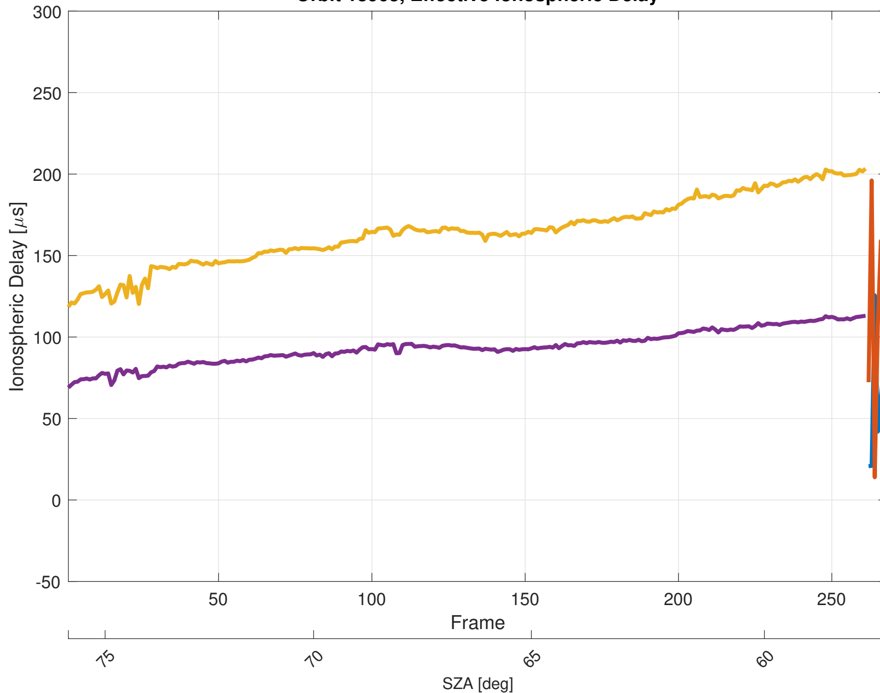
Orbit 18963, Effective Ionospheric Delay
