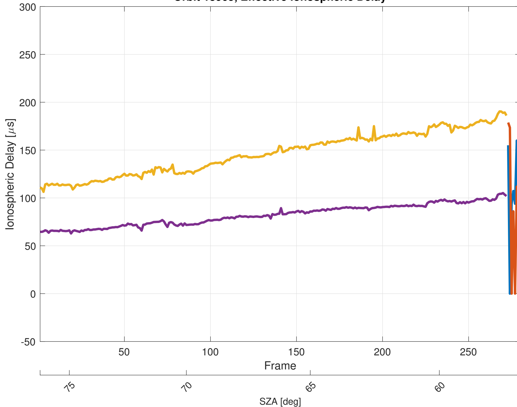
Orbit 18965, Effective Ionospheric Delay
