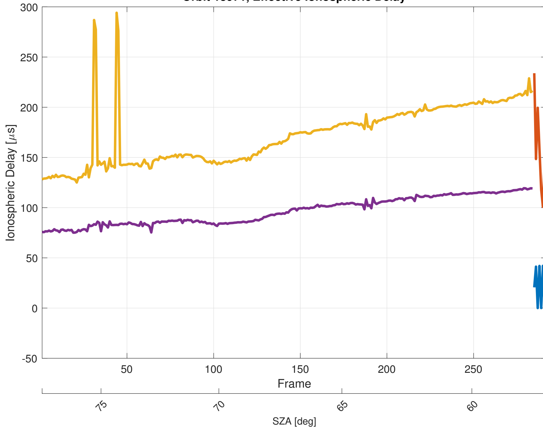
Orbit 18971, Effective Ionospheric Delay
