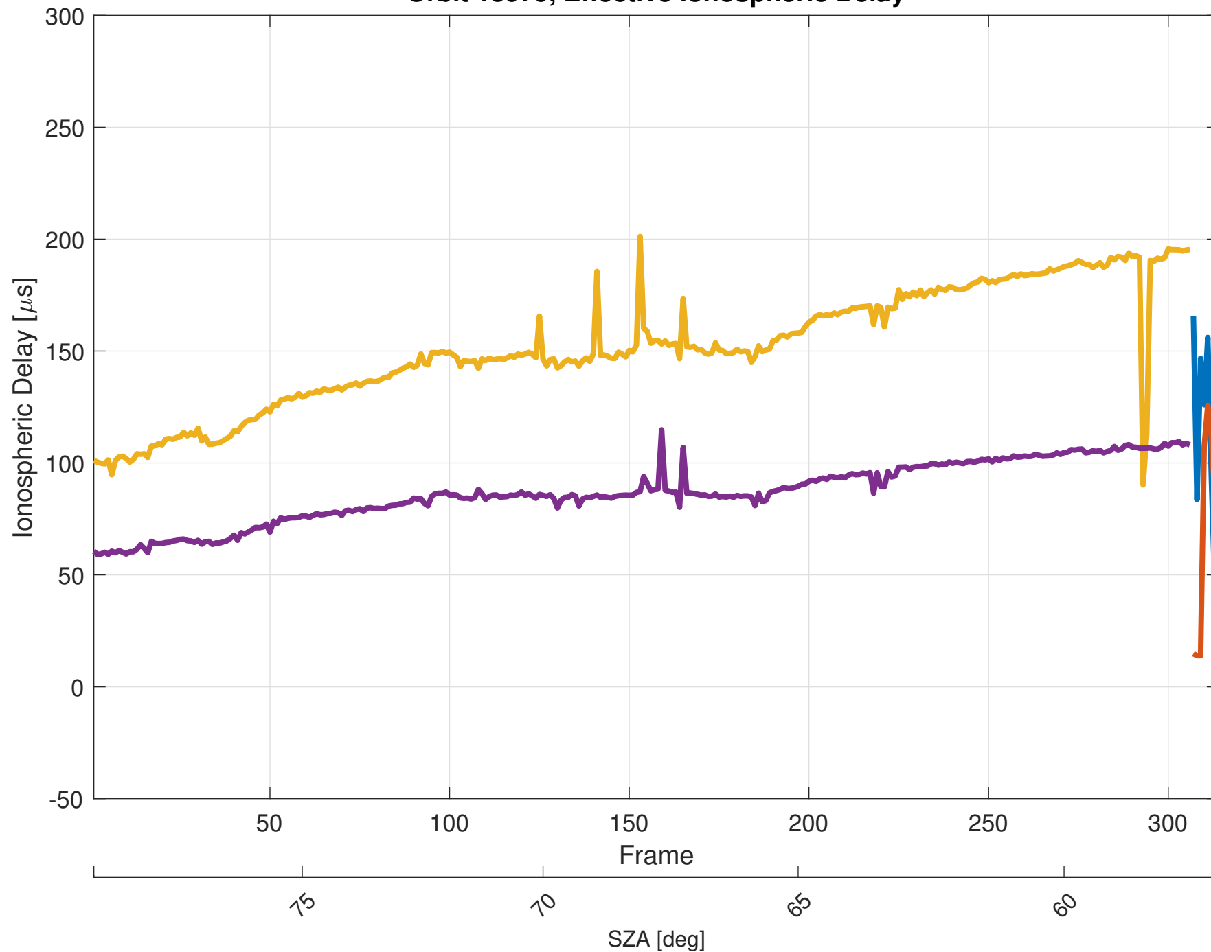
Orbit 18979, Effective Ionospheric Delay
