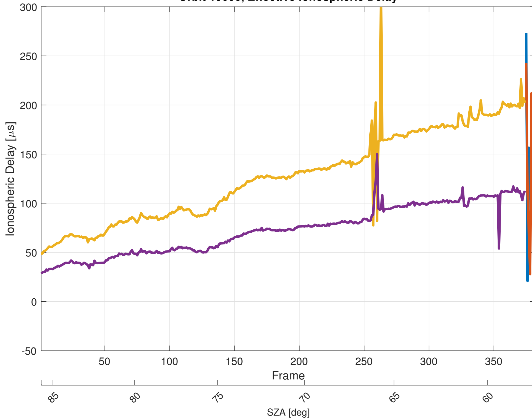
Orbit 19006, Effective Ionospheric Delay
