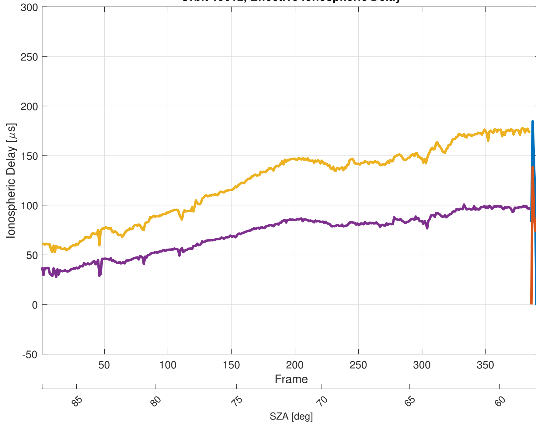
Orbit 19012, Effective Ionospheric Delay
