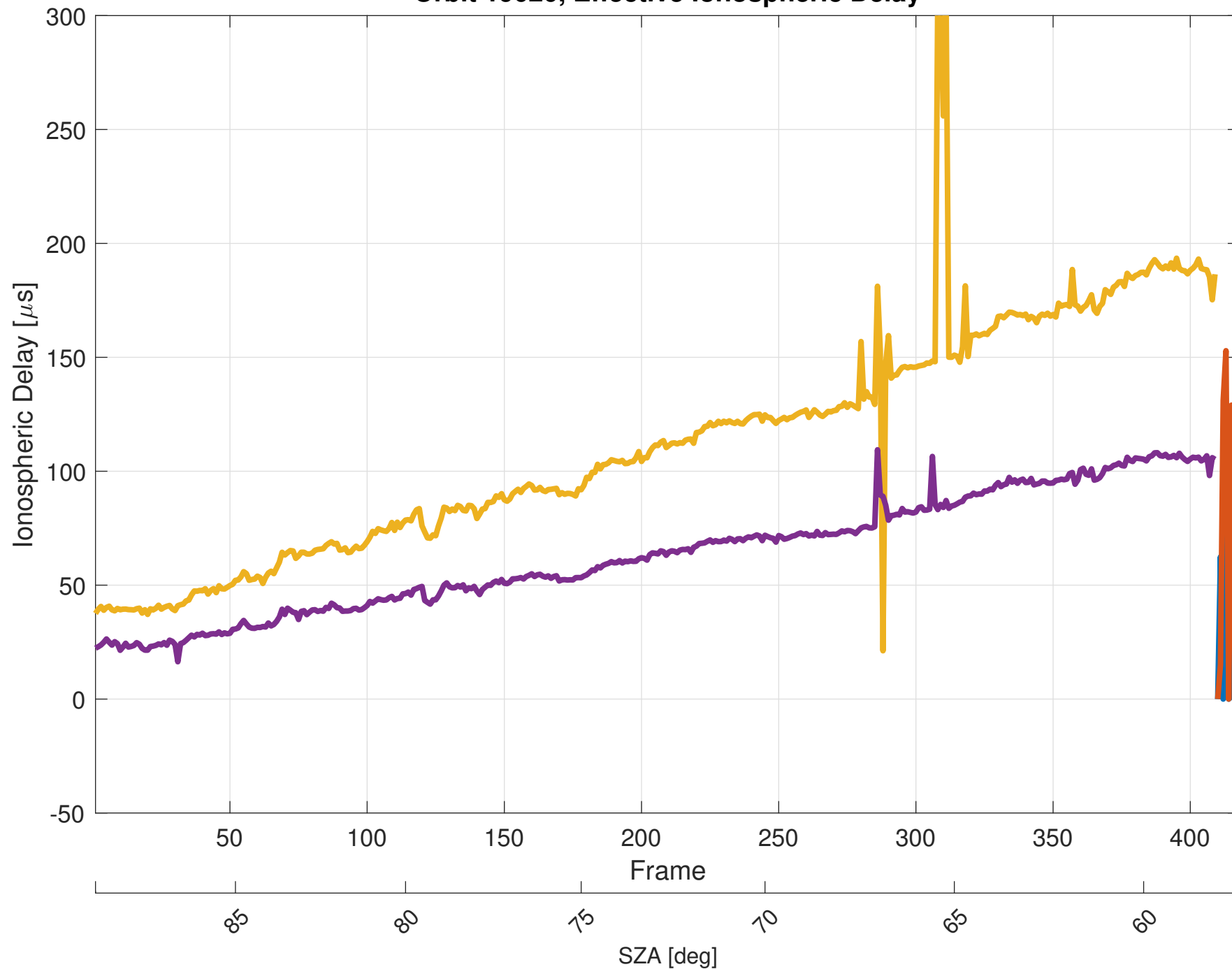
Orbit 19020, Effective Ionospheric Delay
