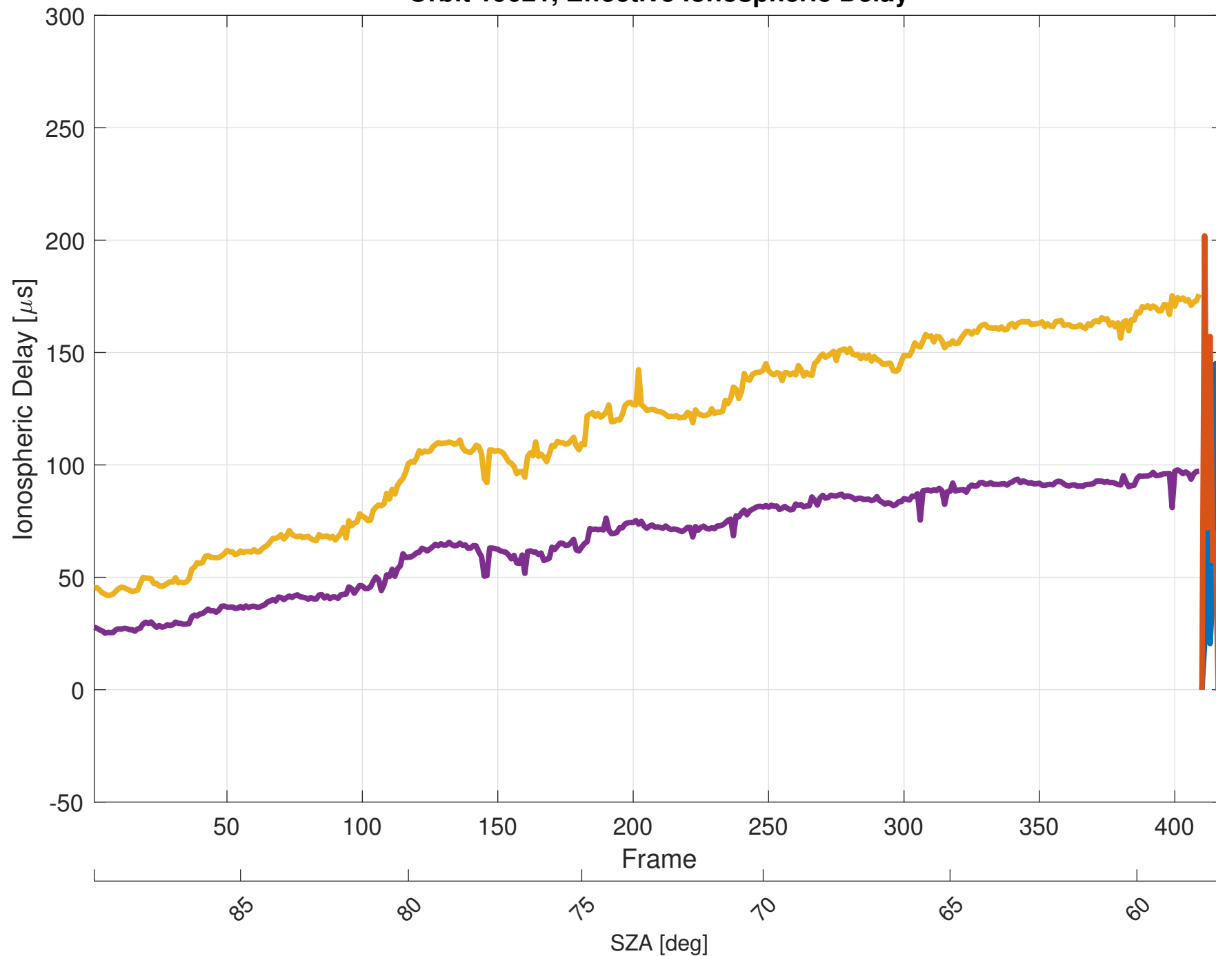
Orbit 19021, Effective Ionospheric Delay
