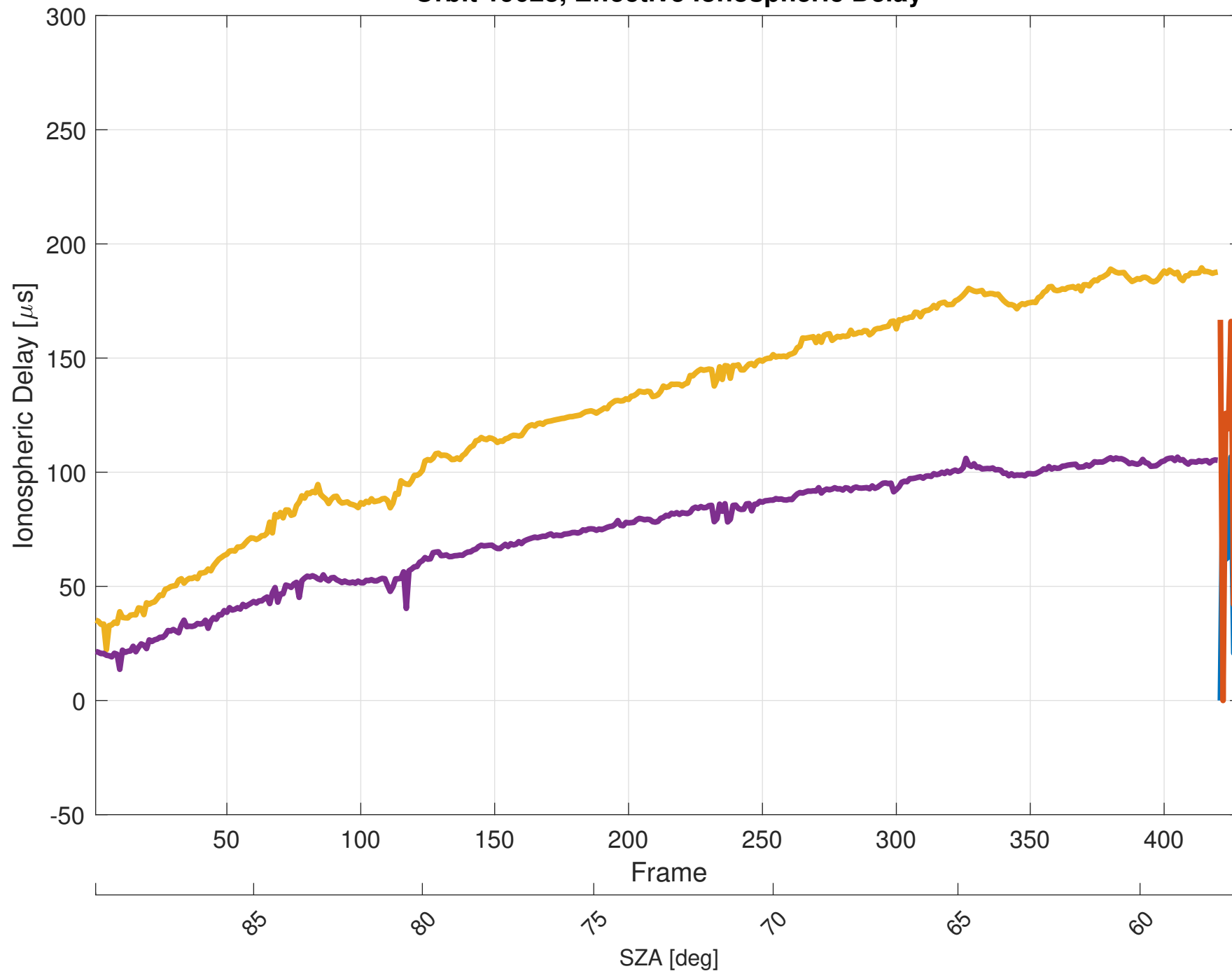
Orbit 19023, Effective Ionospheric Delay
