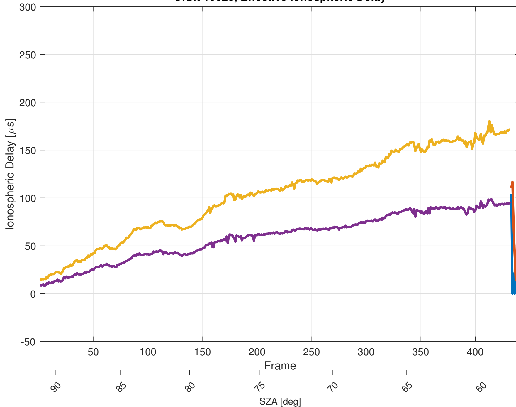
Orbit 19028, Effective Ionospheric Delay
