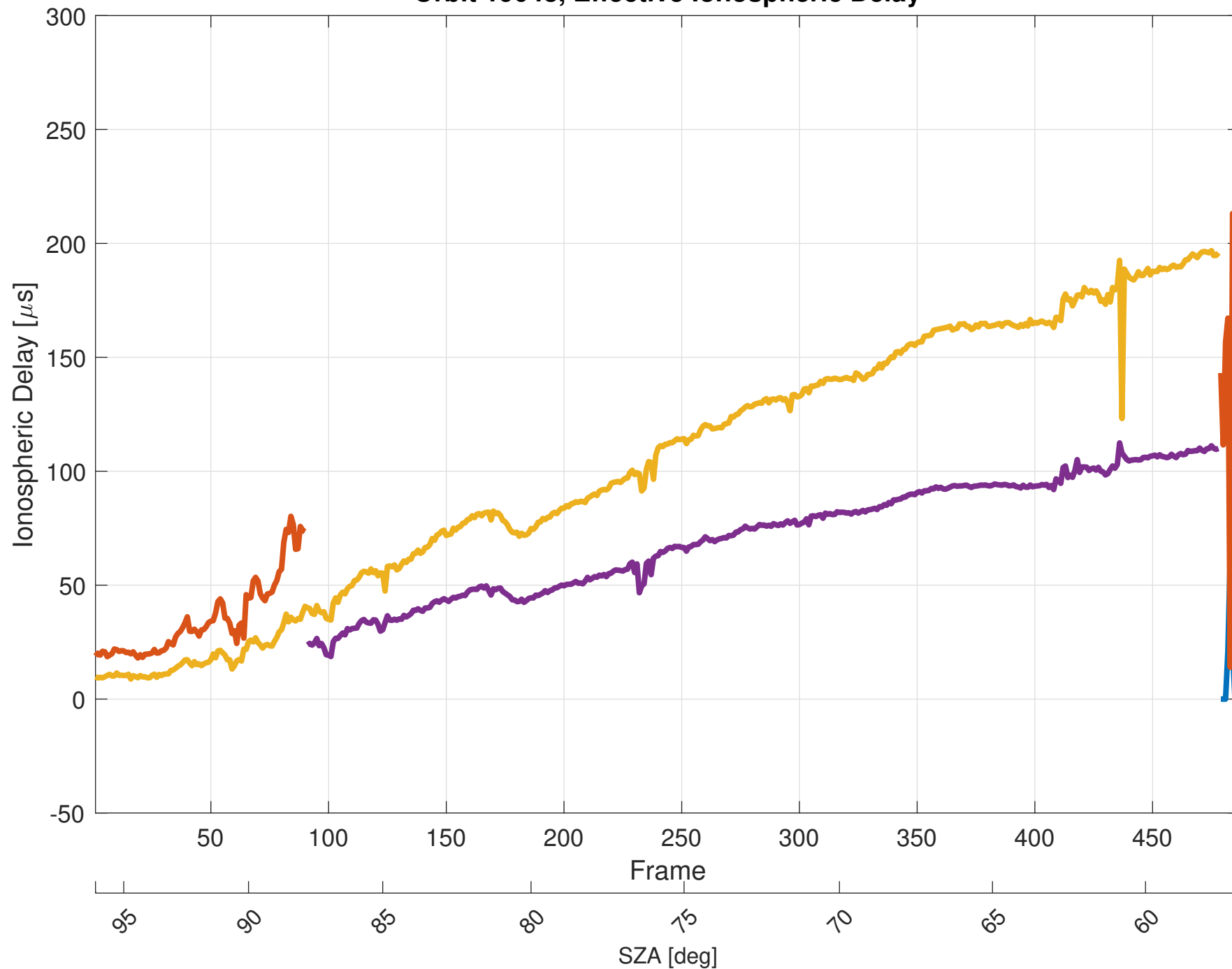
Orbit 19048, Effective Ionospheric Delay
