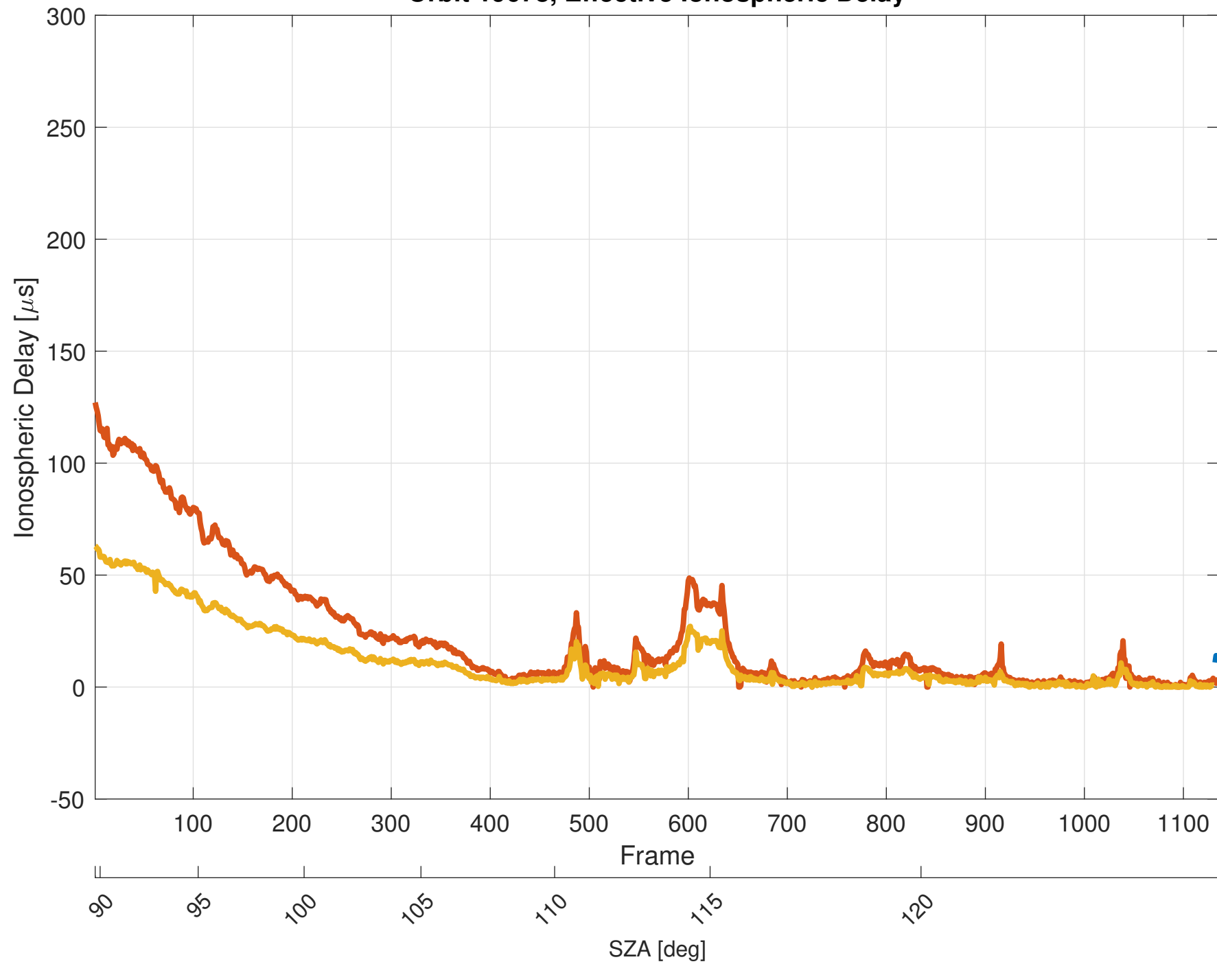
Orbit 19678, Effective Ionospheric Delay
