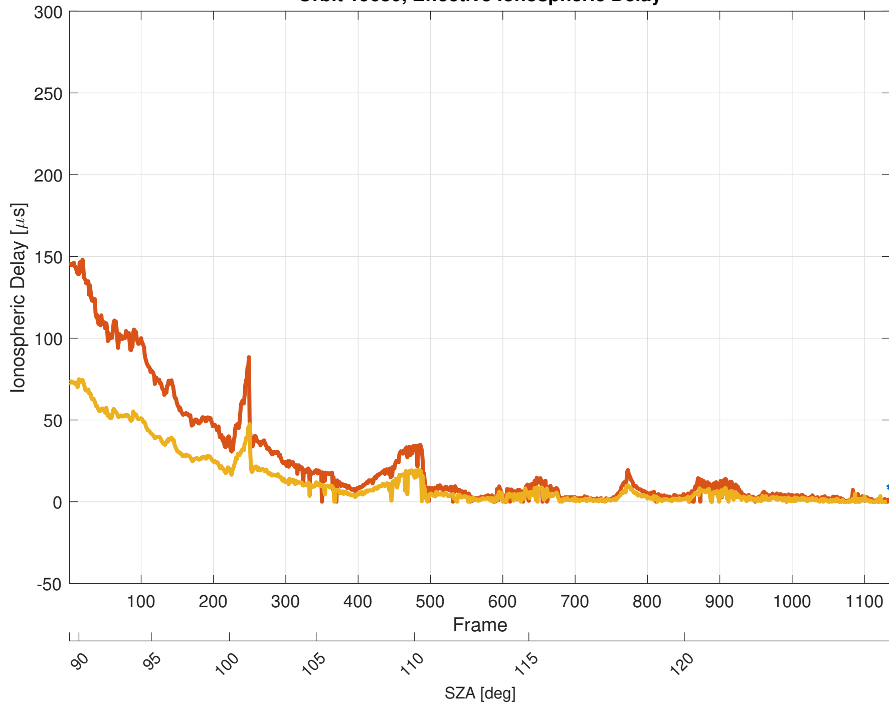
Orbit 19680, Effective Ionospheric Delay
