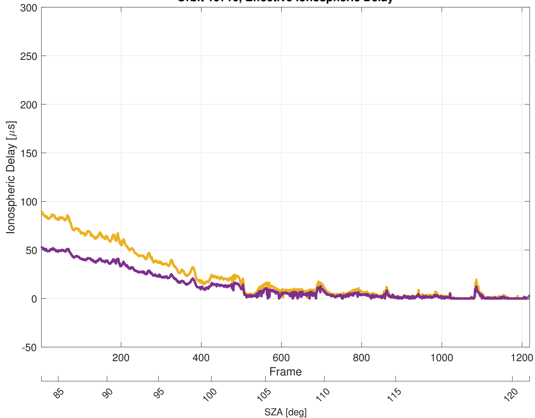
Orbit 19710, Effective Ionospheric Delay
