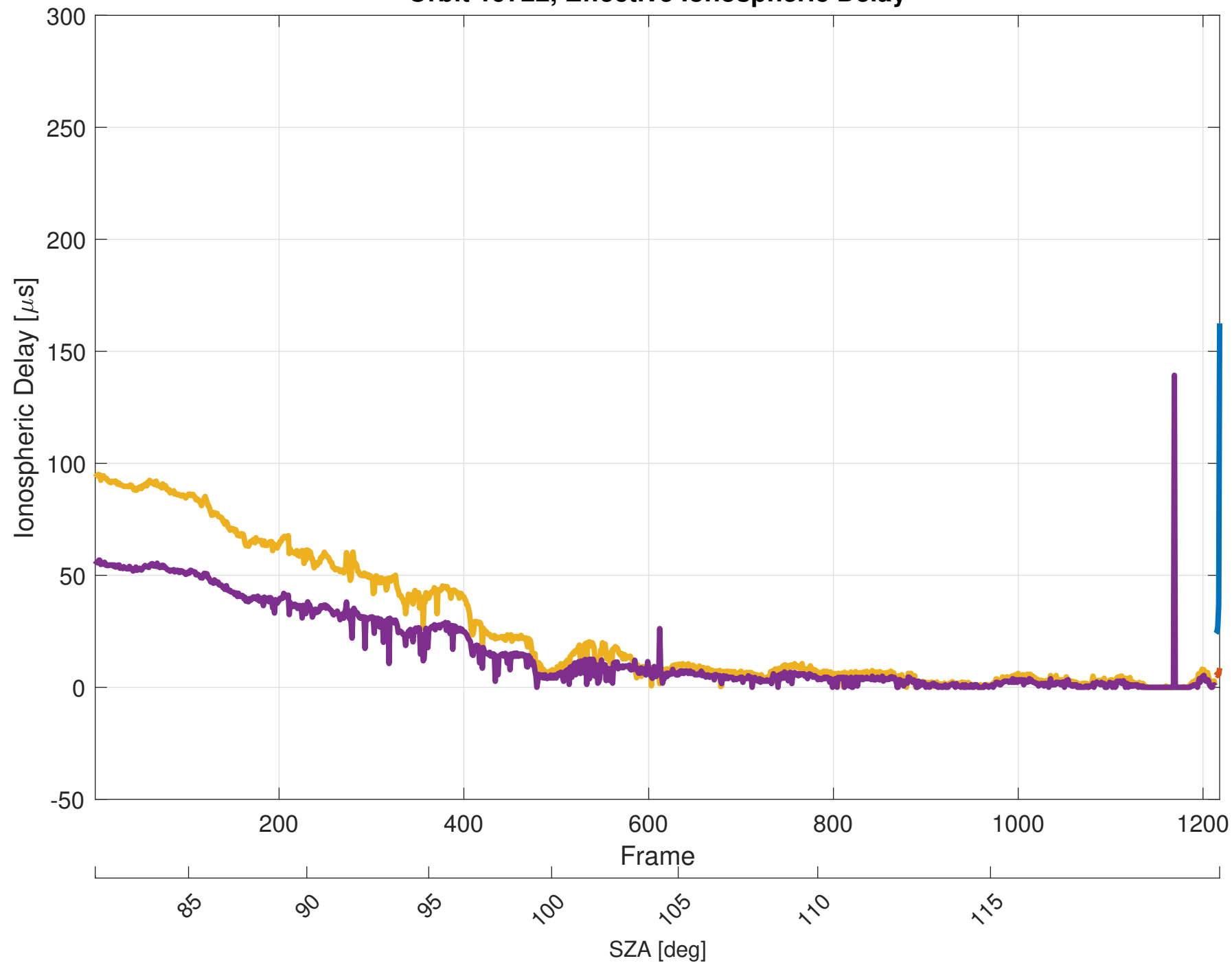
Orbit 19722, Effective Ionospheric Delay
