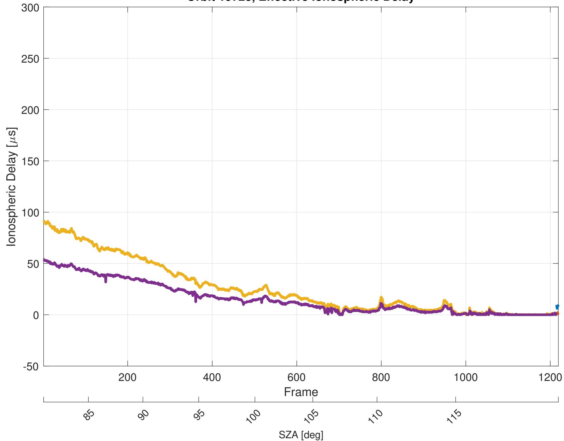
Orbit 19723, Effective Ionospheric Delay
