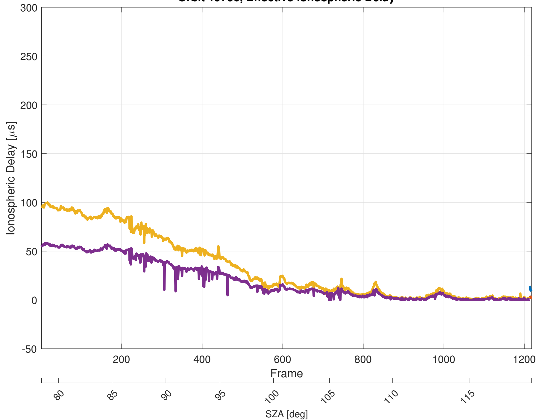
Orbit 19736, Effective Ionospheric Delay
