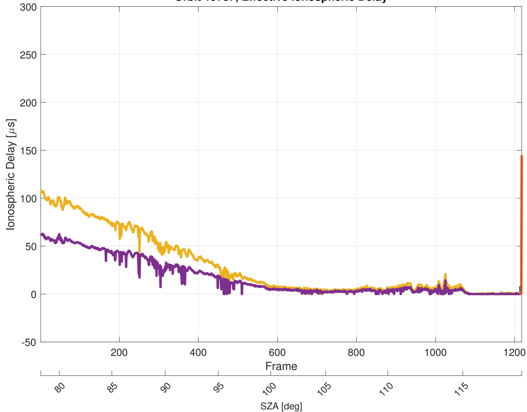
Orbit 19737, Effective Ionospheric Delay
