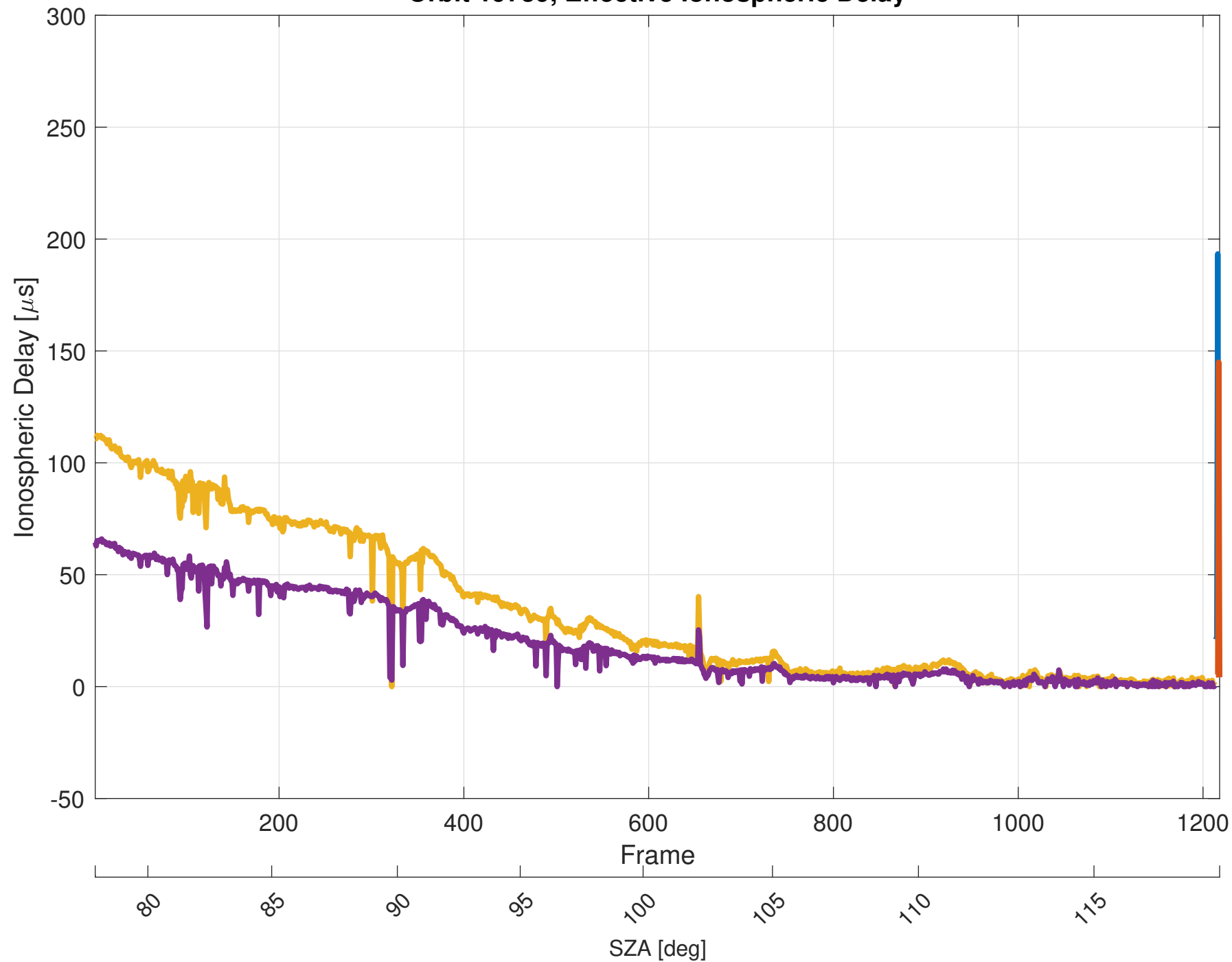
Orbit 19739, Effective Ionospheric Delay
