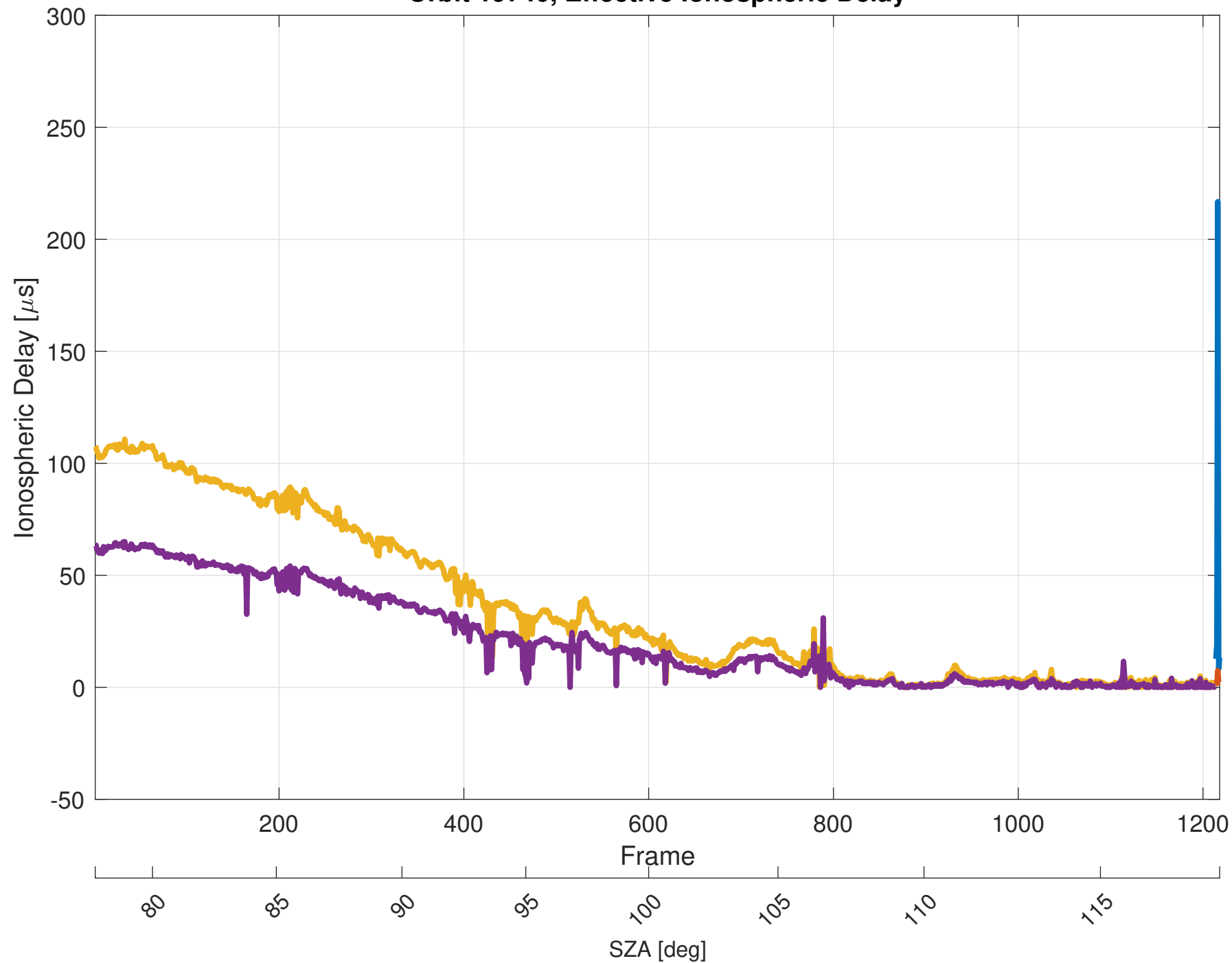
Orbit 19740, Effective Ionospheric Delay
