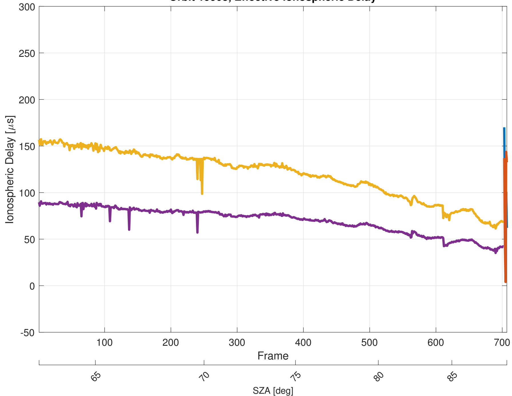
Orbit 19903, Effective Ionospheric Delay
