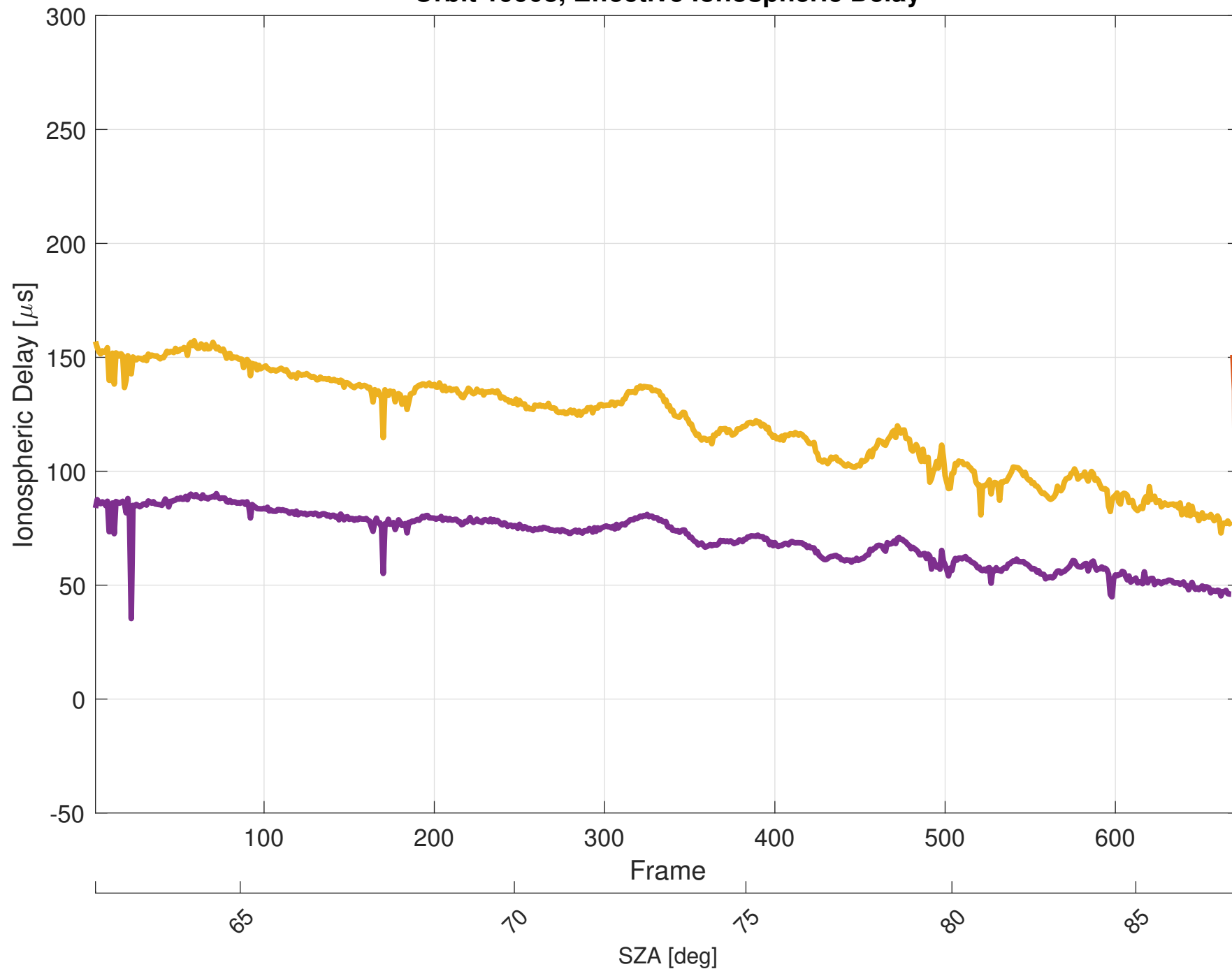
Orbit 19908, Effective Ionospheric Delay
