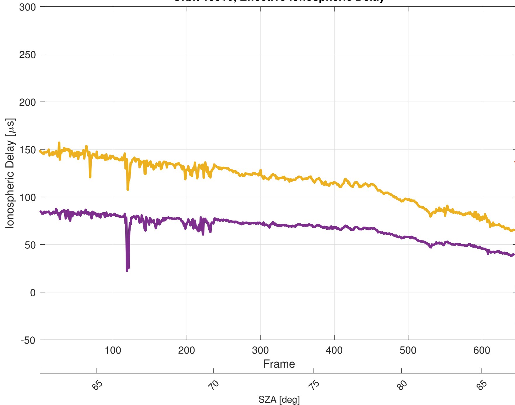
Orbit 19910, Effective Ionospheric Delay
