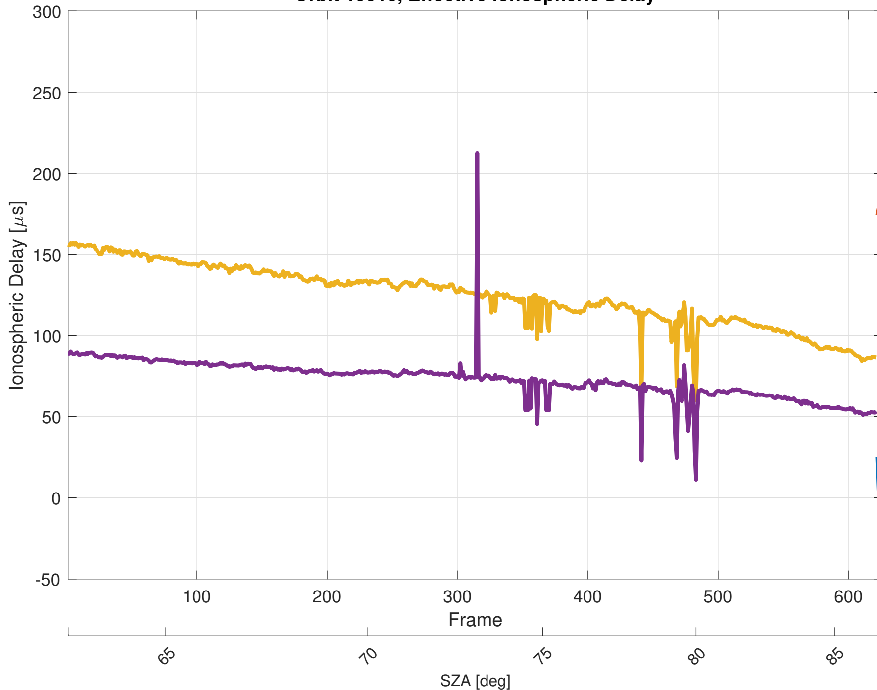
Orbit 19913, Effective Ionospheric Delay
