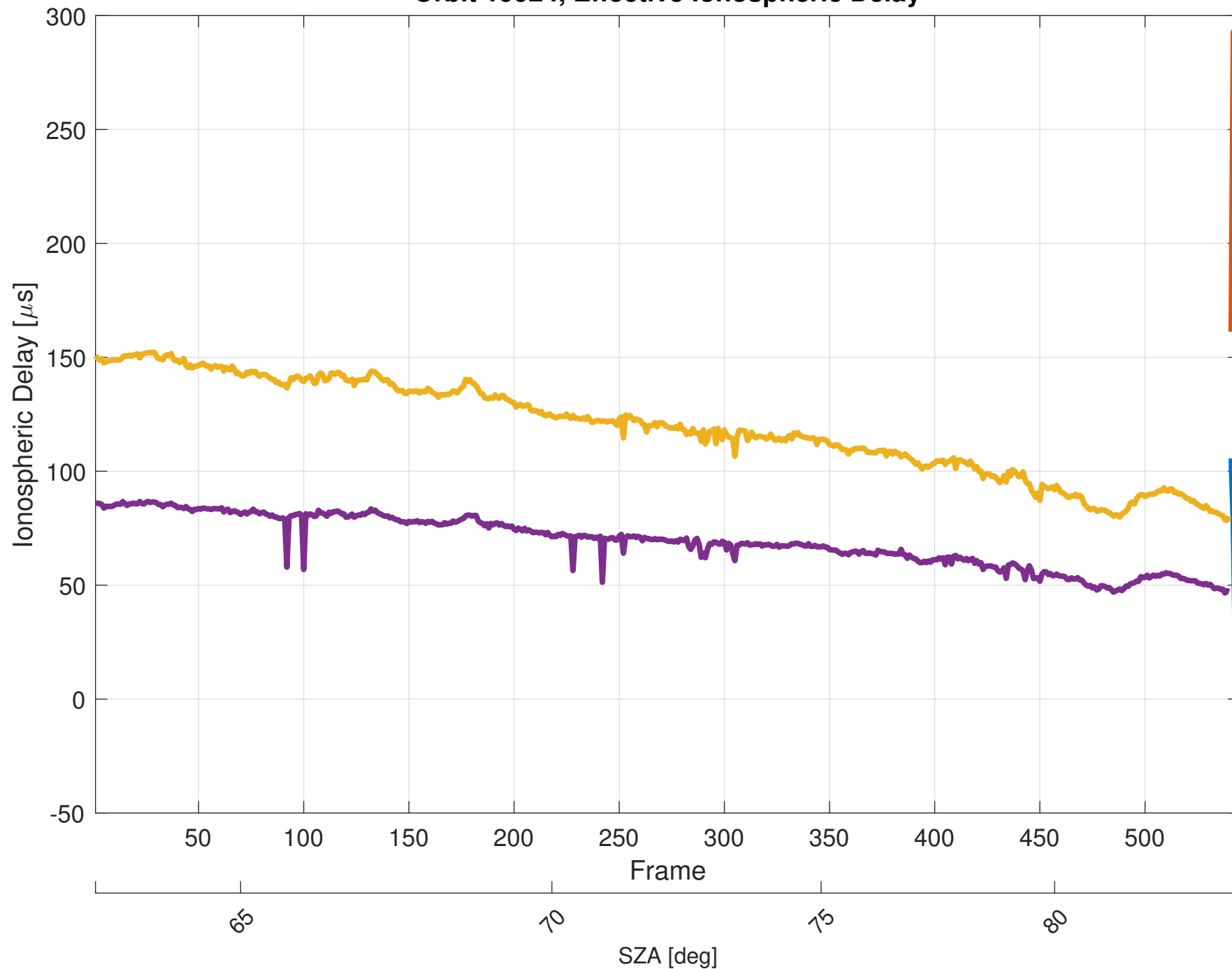
Orbit 19924, Effective Ionospheric Delay
